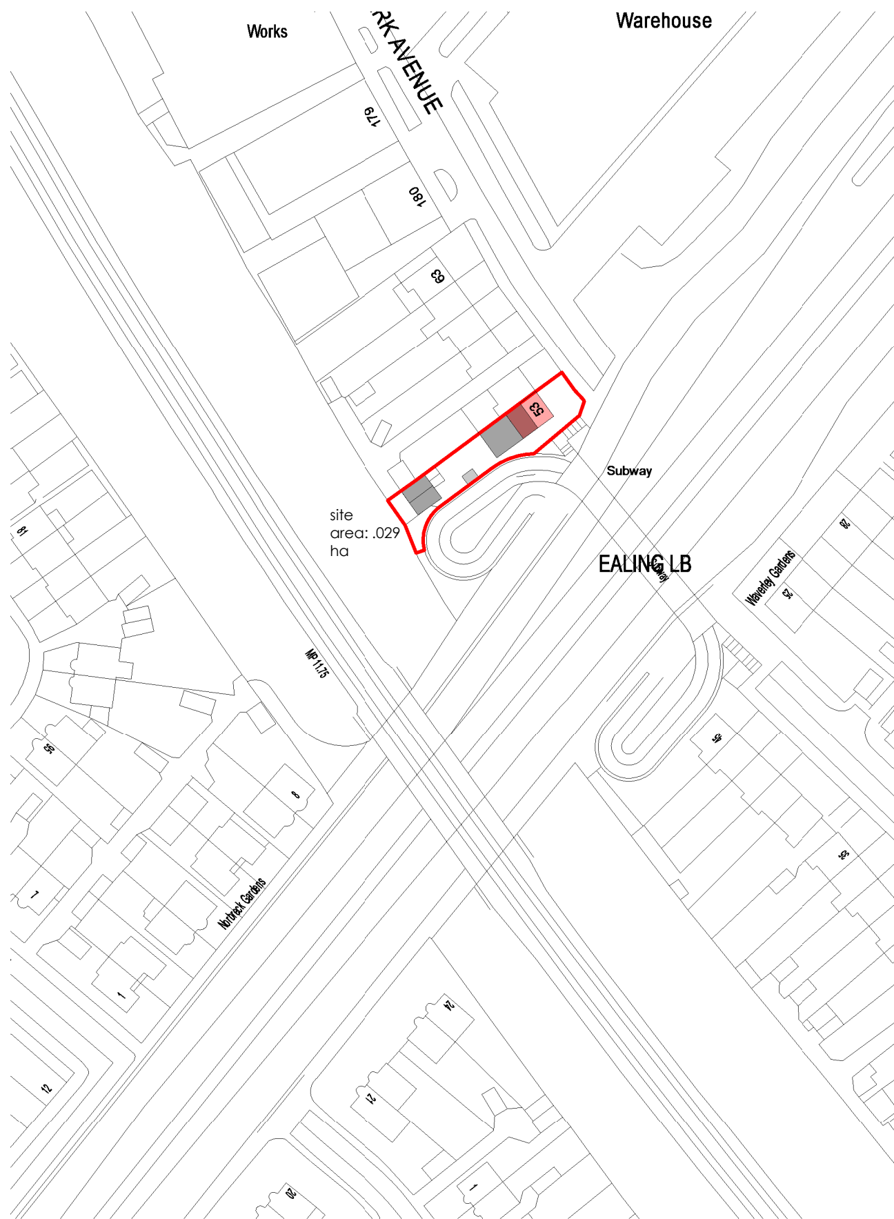
1 Location Plan 2314-L-100 1 : 1000
