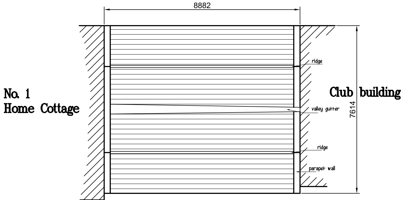
ROOF PLAN – scale 1:100 STONELEIGH CLUB VICARAGE ROAD, STONELEIGH
