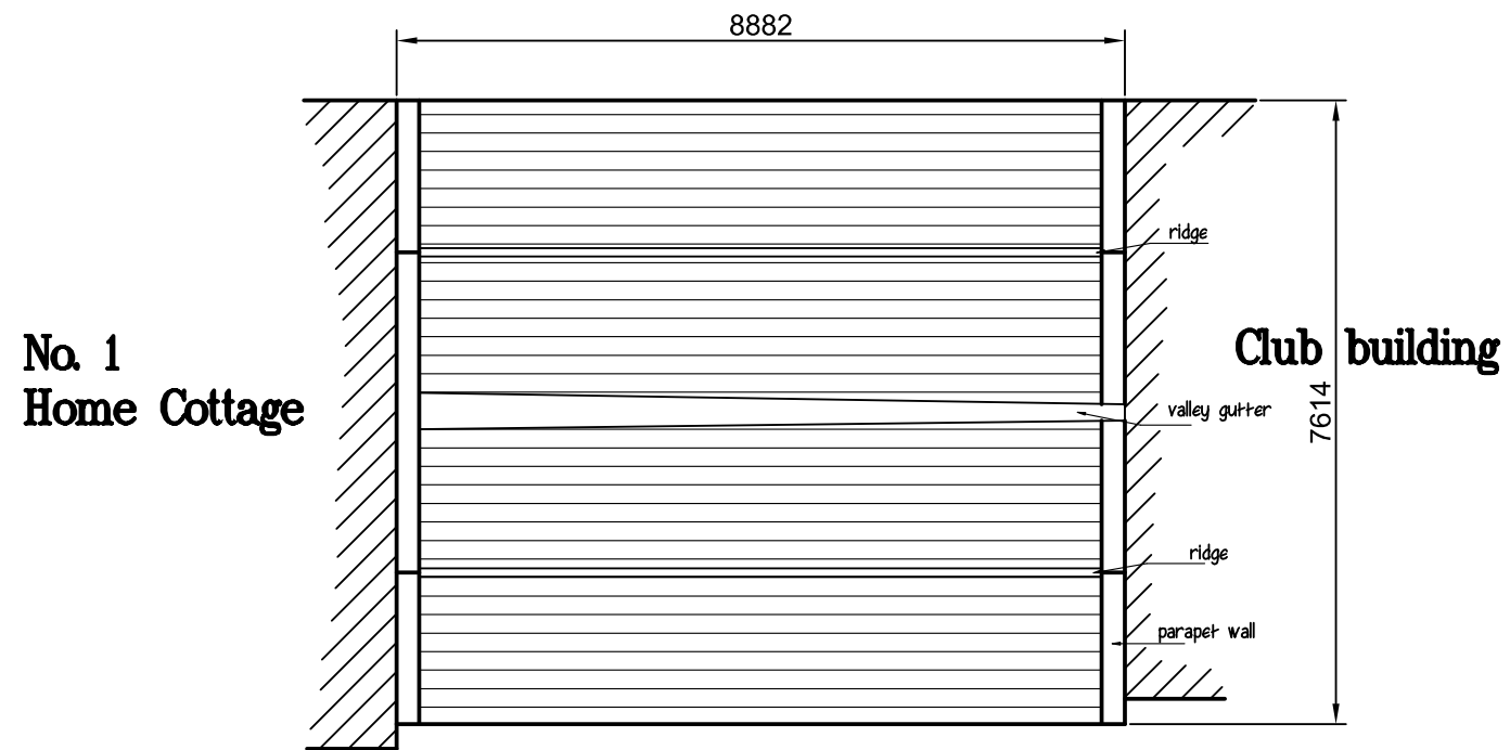
EXISTING ROOF PLAN – scale 1:100 @ A4 STONELEIGH CLUB VICARAGE ROAD, STONELEIGH
