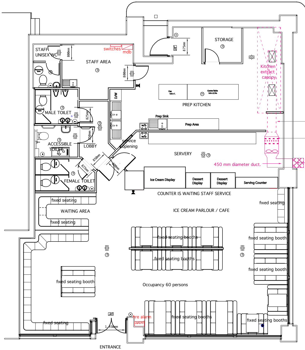
PLAN AS PROPOSED Scale 1: 100
