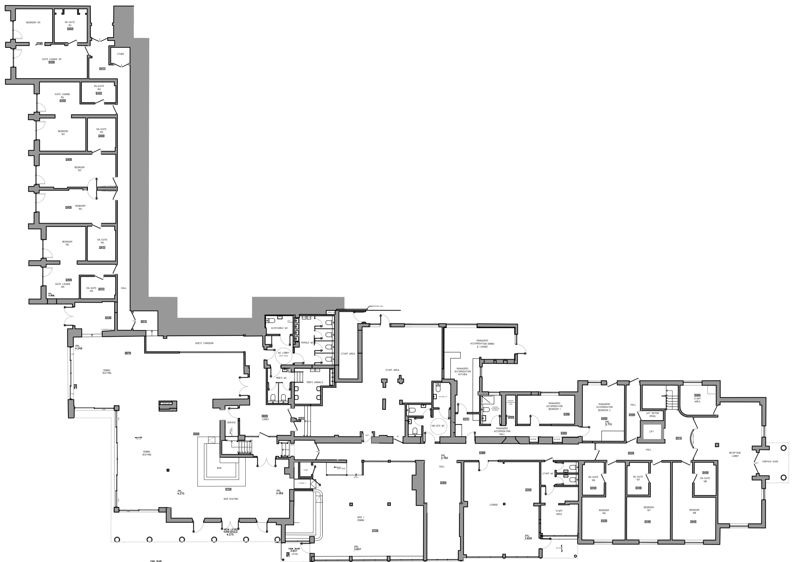
PROPOSED GF PLAN SCALE 1:200 @ A1
