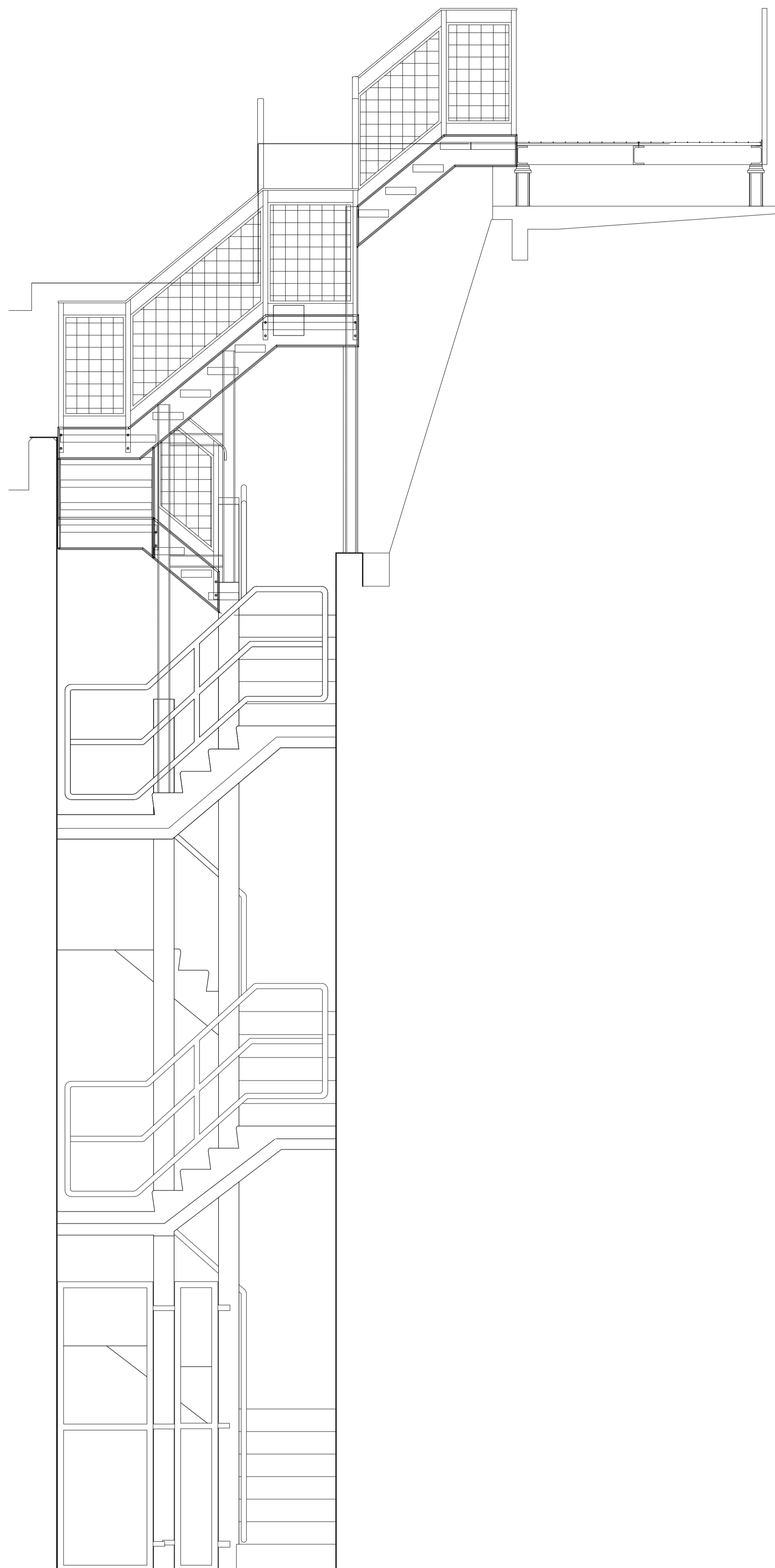
01 Existing Fire Escape Stair Elevation (Approved) 10.272 1:25@A1, 1:50@A3
