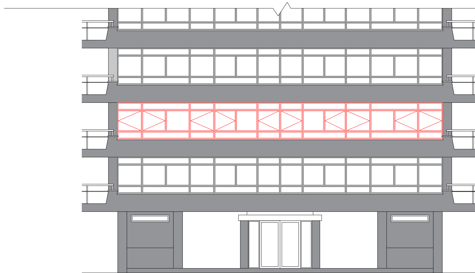
EXISTING FRONT ELEVATION (SOUTH EAST)
