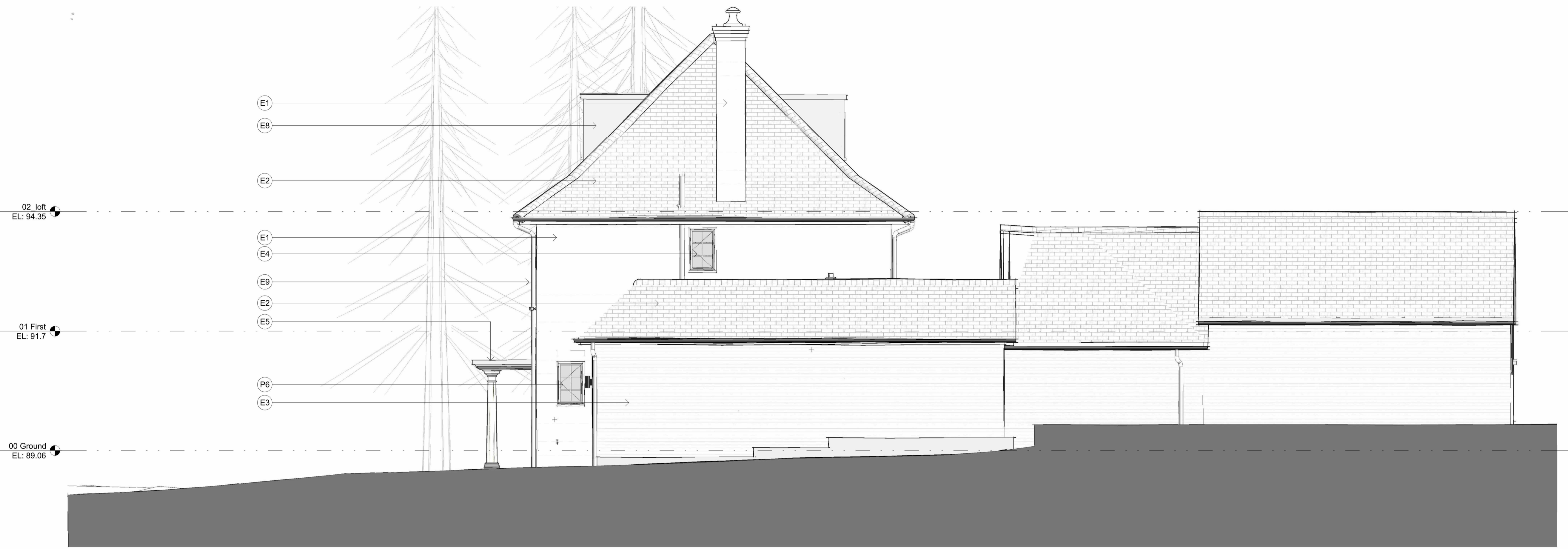
1 North West Elevation - Existing 3010 1:50
