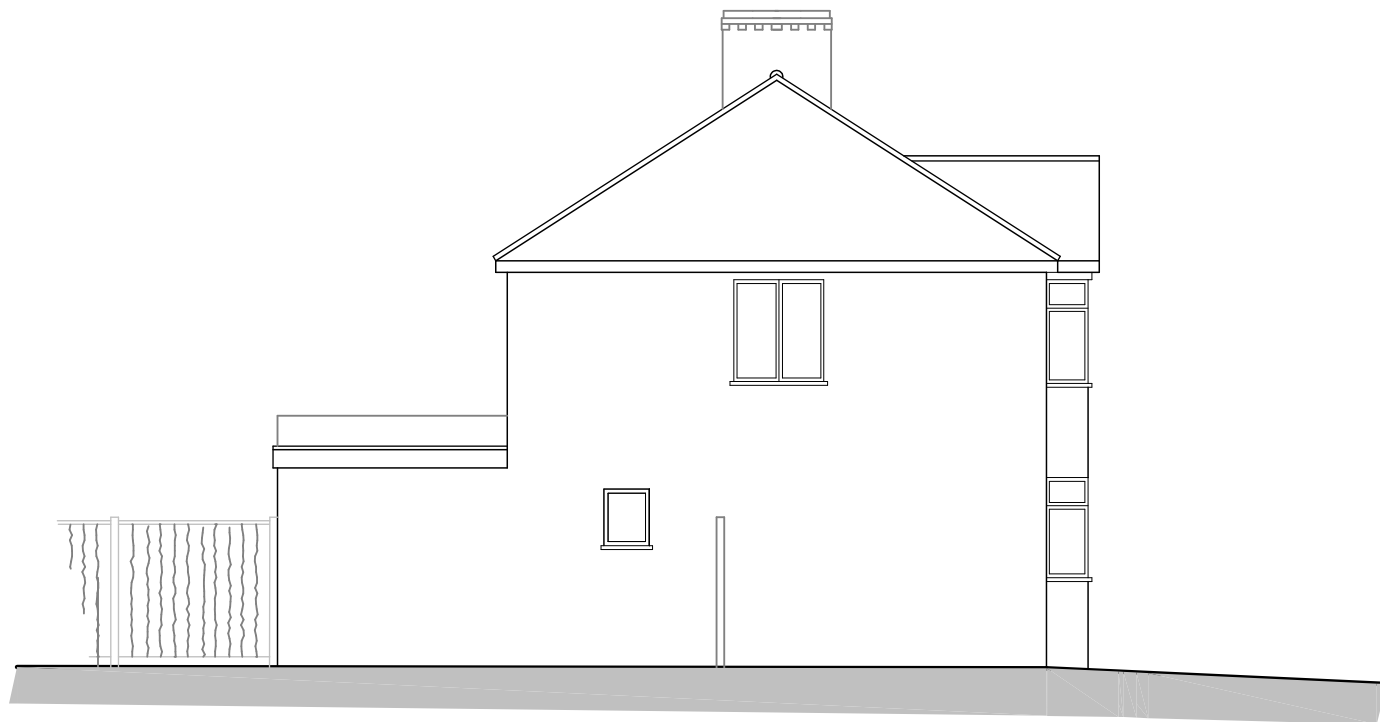
SIDE ELEVATION WESTERN
