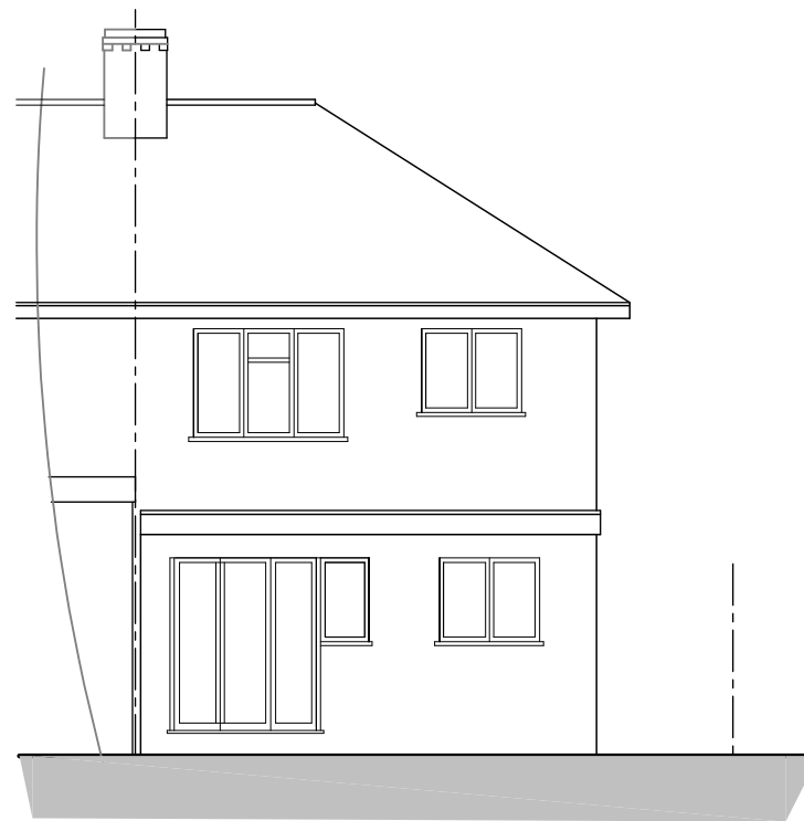
REAR ELEVATION NORTHERN
