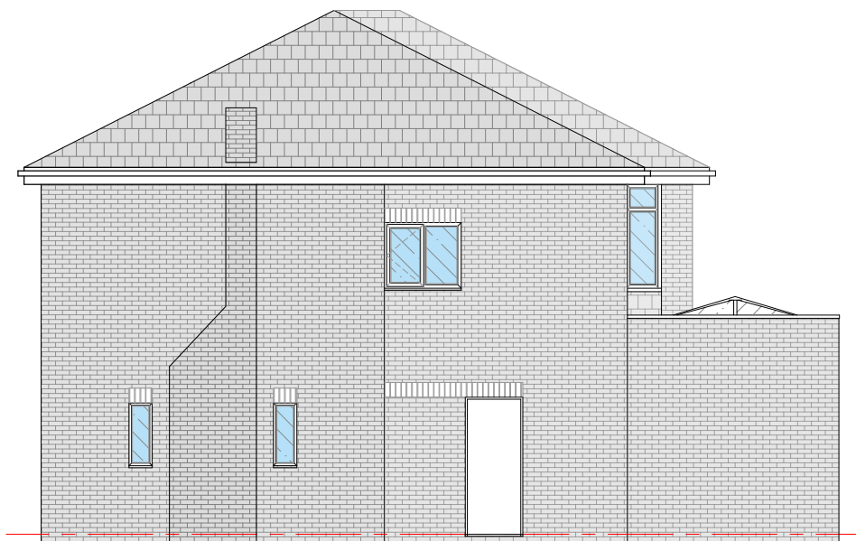
Proposed Left Side Elevation (Scale - 1:100)
