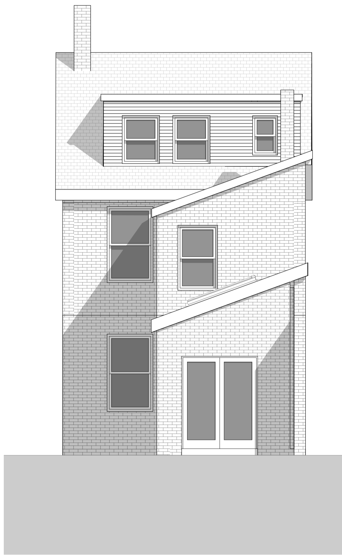
B 2 N-02 North Elevation 1:50
