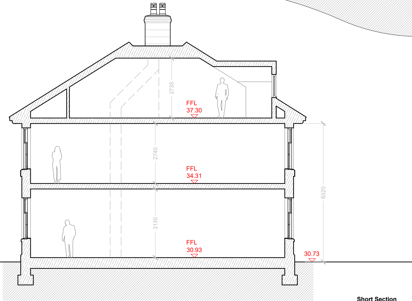
Short Section 1:100
