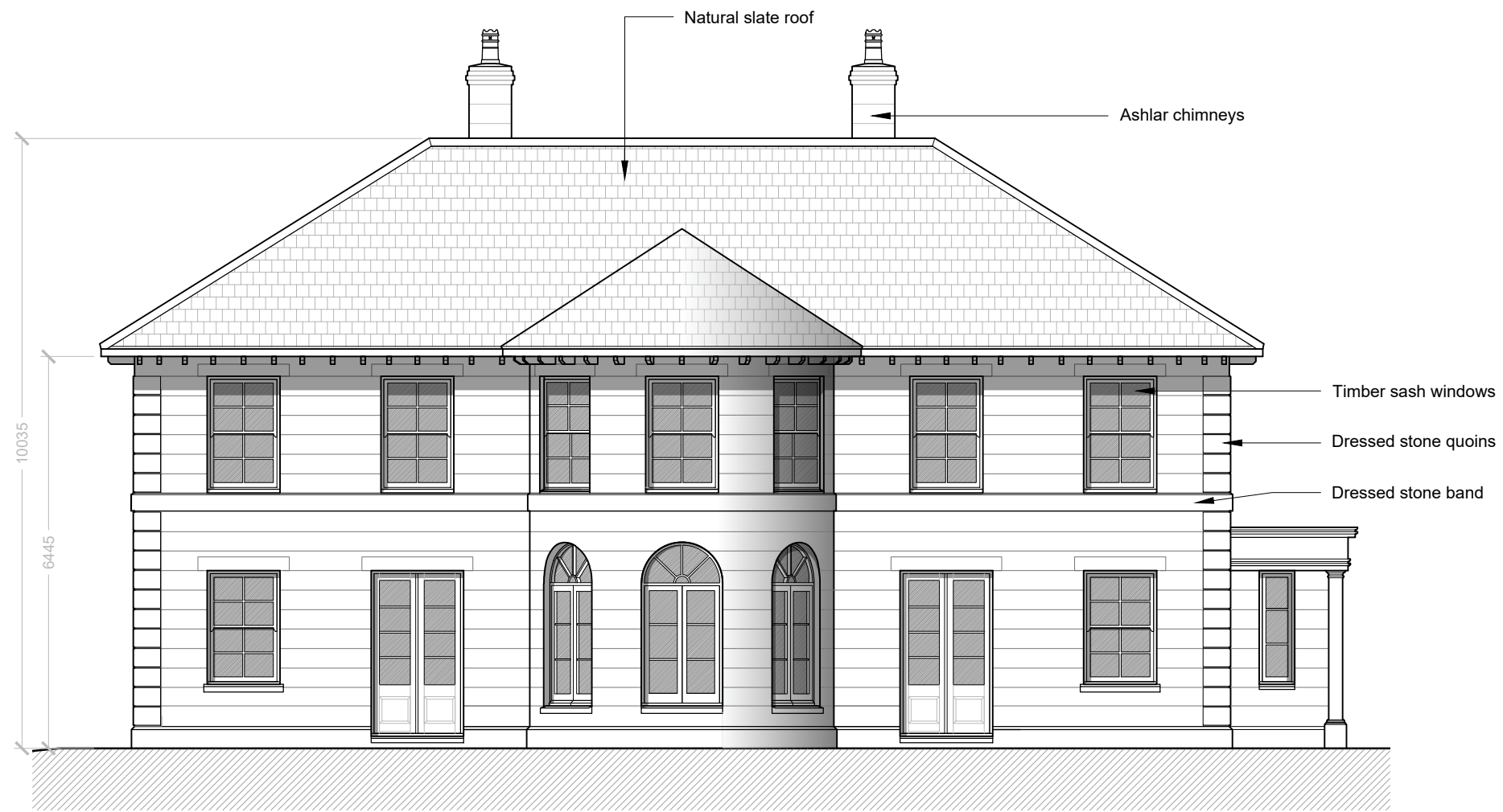
North Elevation 1:100
