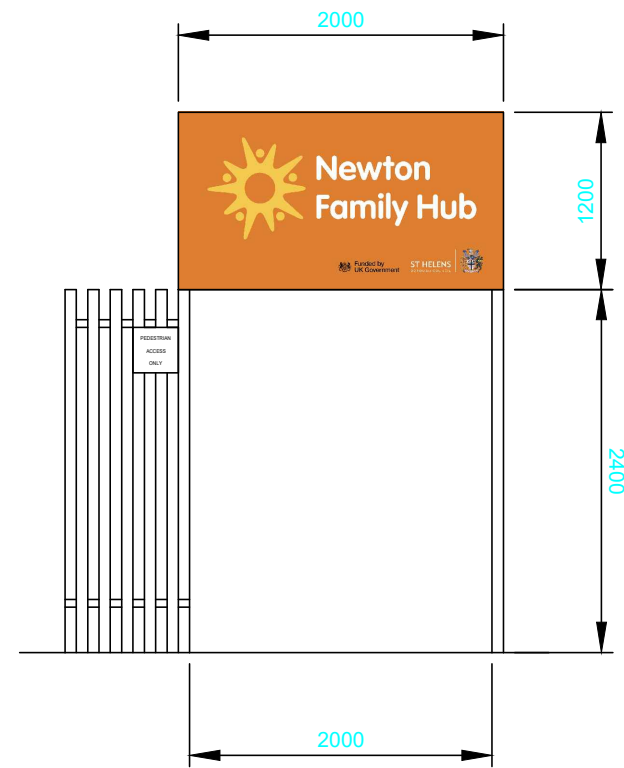
PROPOSED FENCE MOUNTED SIGN
