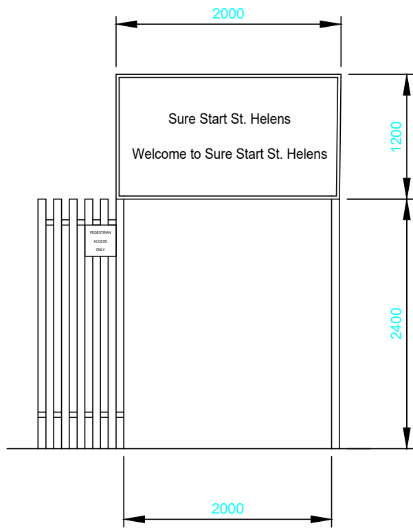
EXISTING FENCE MOUNTED SIGN
