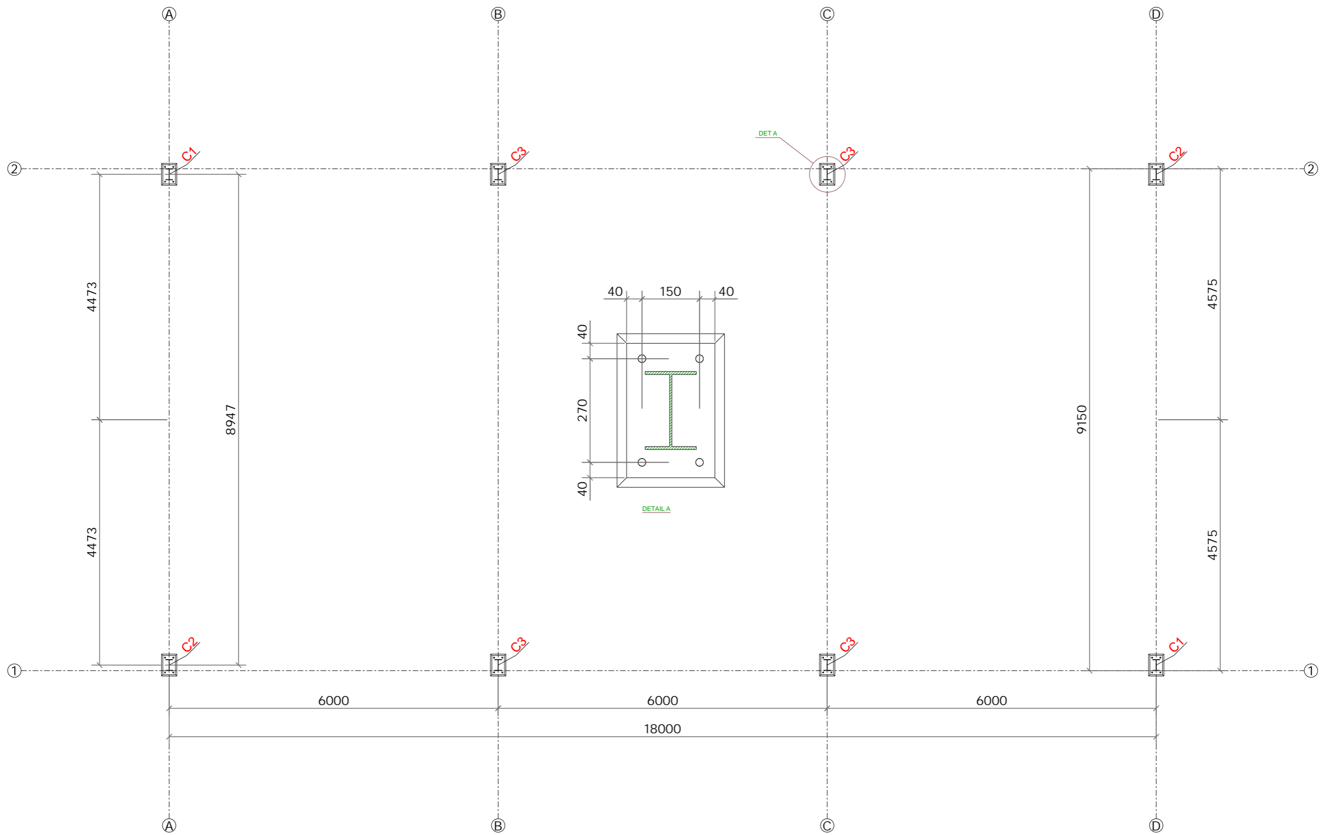
Plan on Foundations
