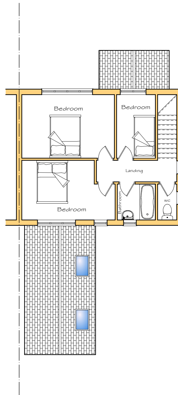
First Floor as Proposed.
