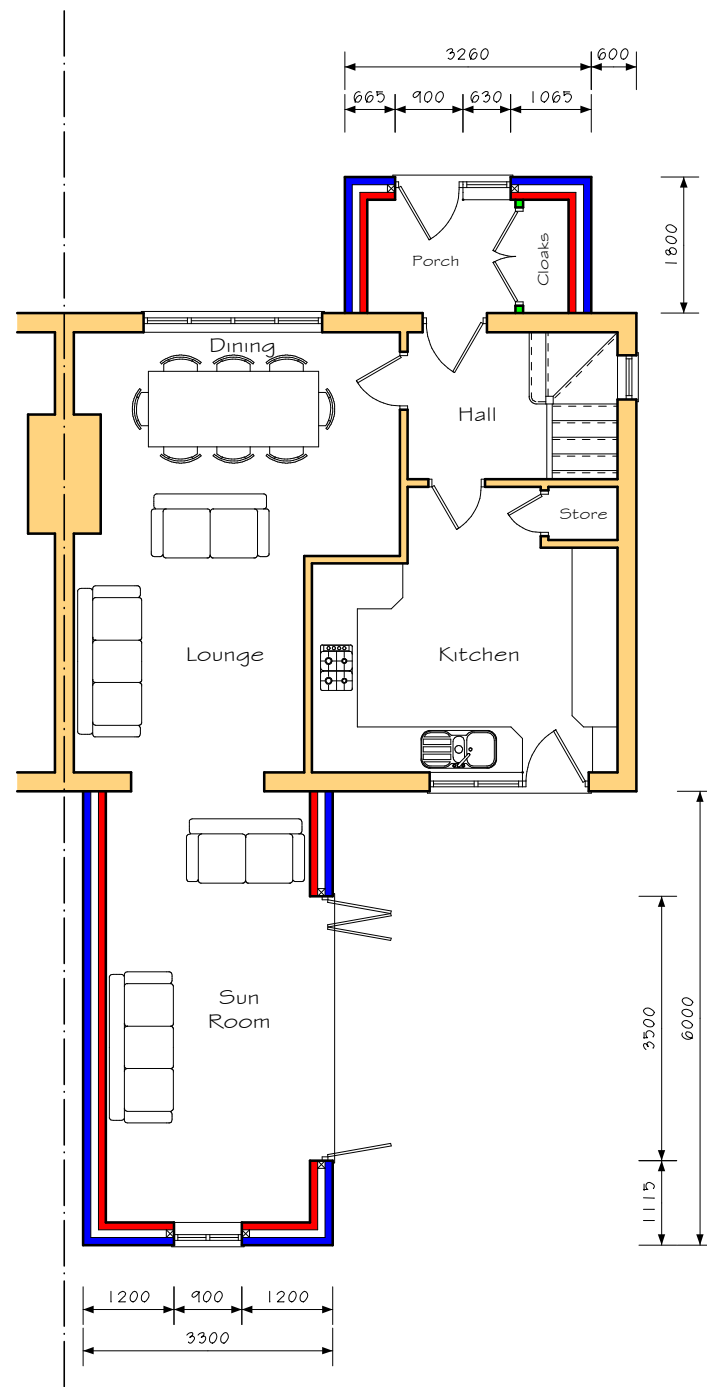
Ground Floor as Proposed.
