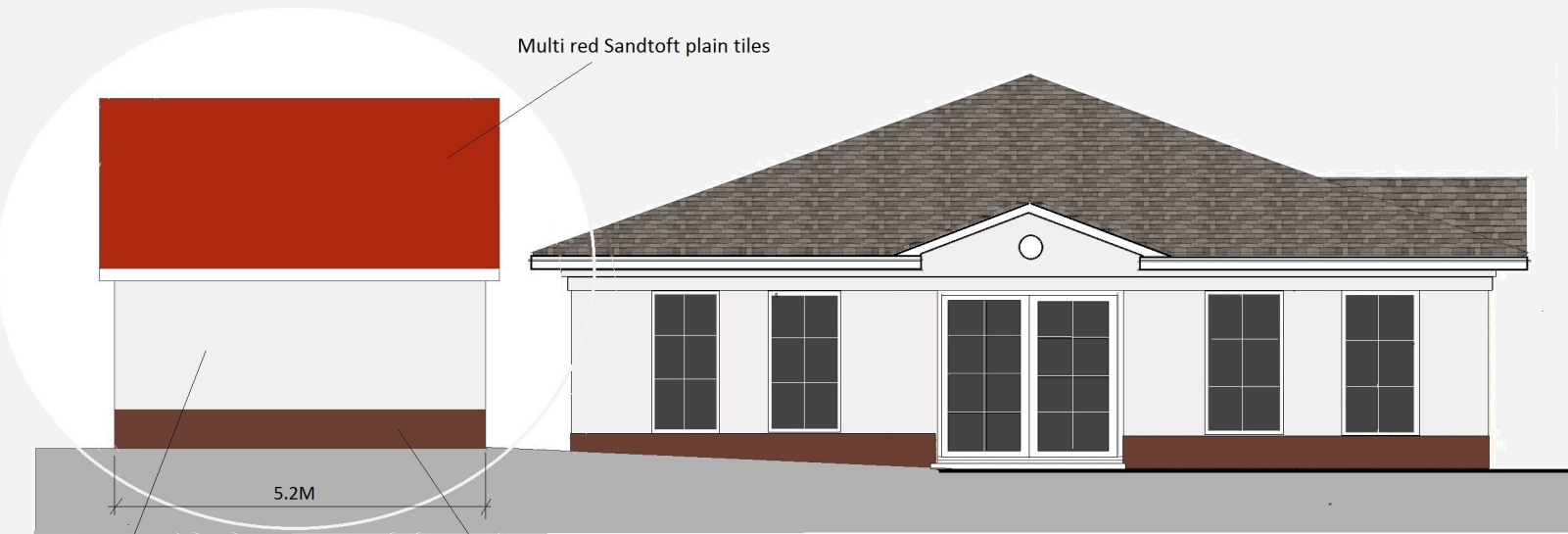
North elevation
