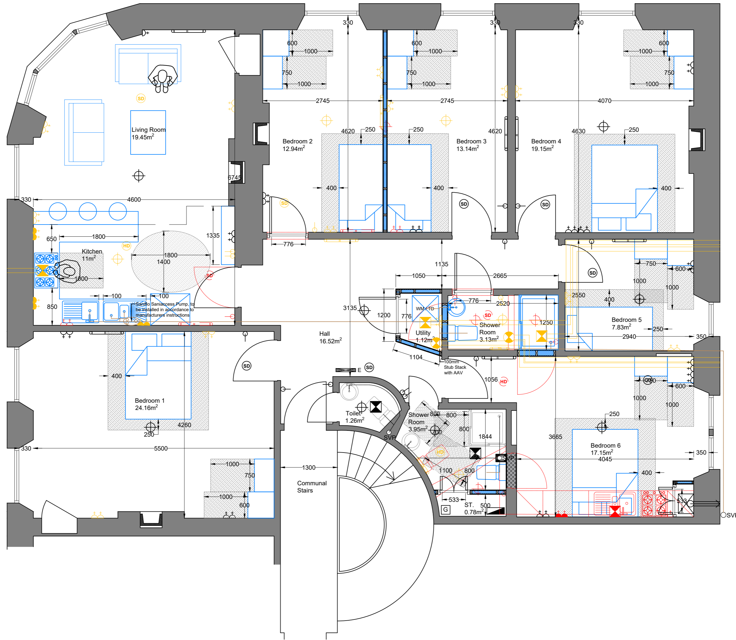
Proposed Floor Plan 1:50
