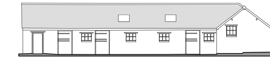
Barn A - West Elevation
