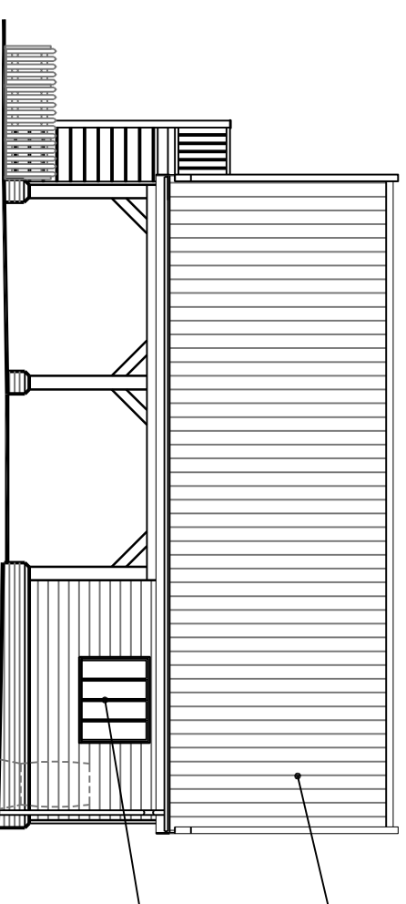
south-west elevation
