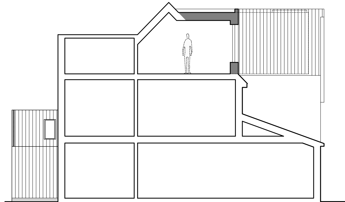
1 proposed section scale 1:100 @ A3
