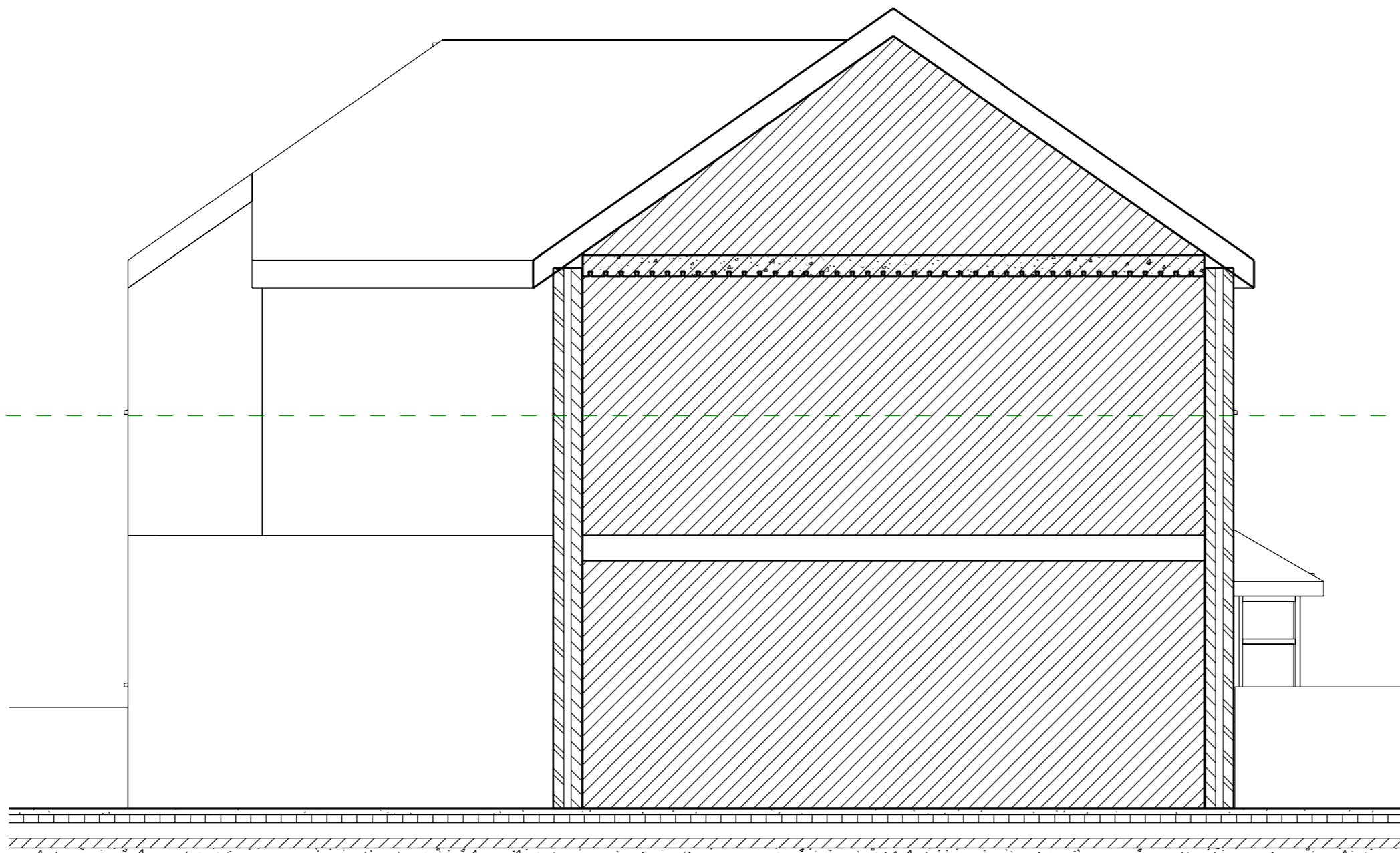
1 Proposed Elevation viewed from no.57 1 : 50
