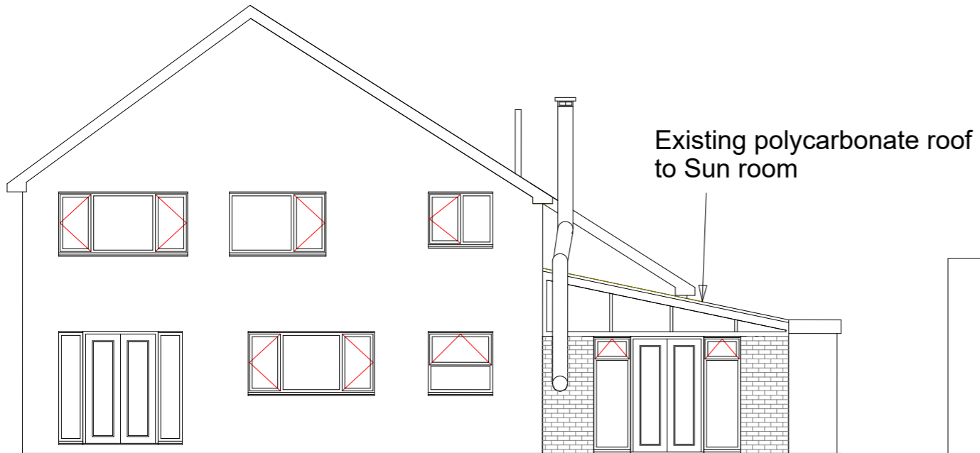
Rear Elevation
