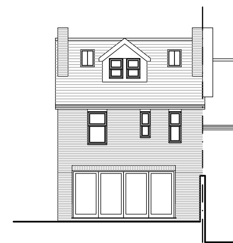
REAR ELEVATION (NORTH)
