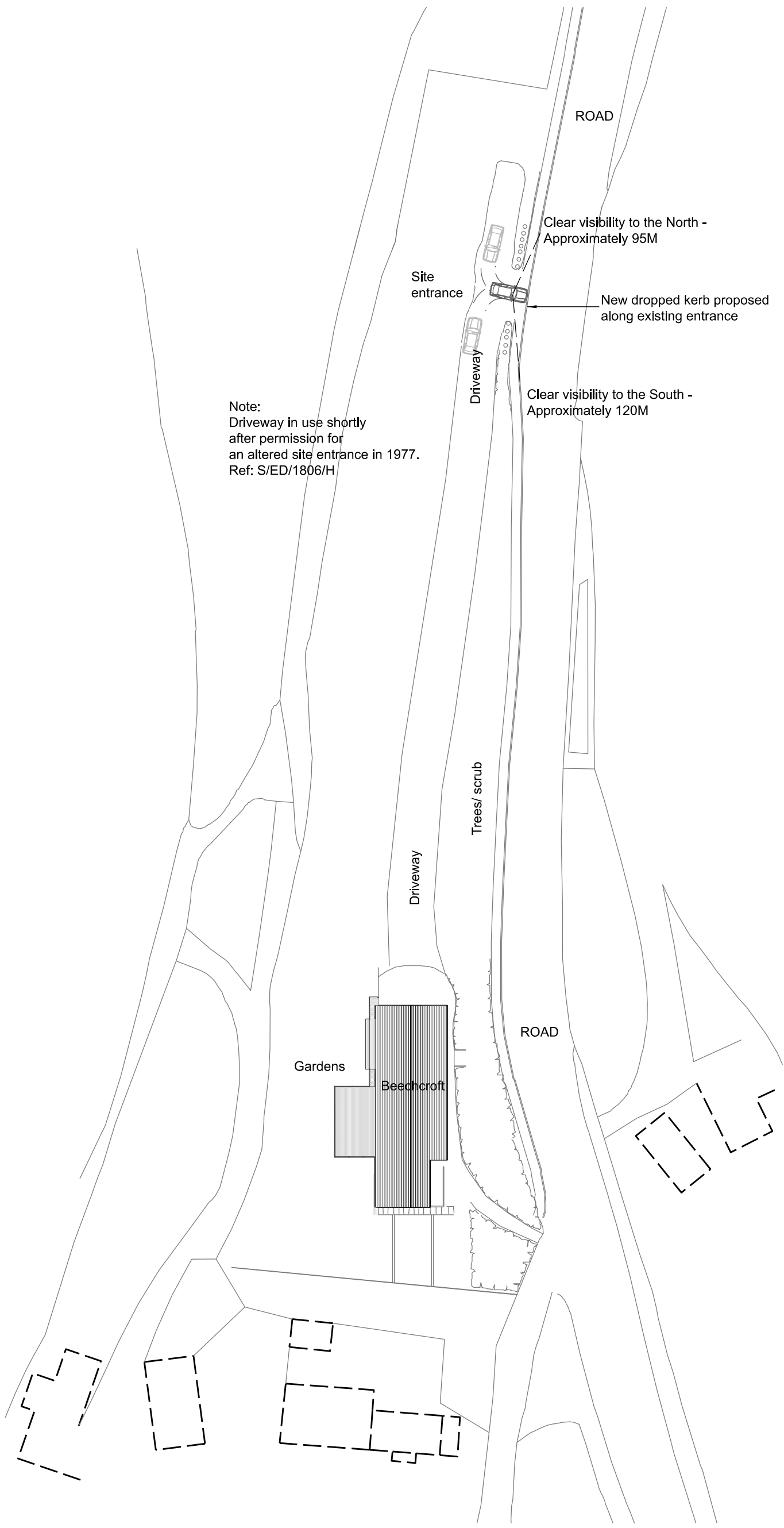
SITE PLAN
