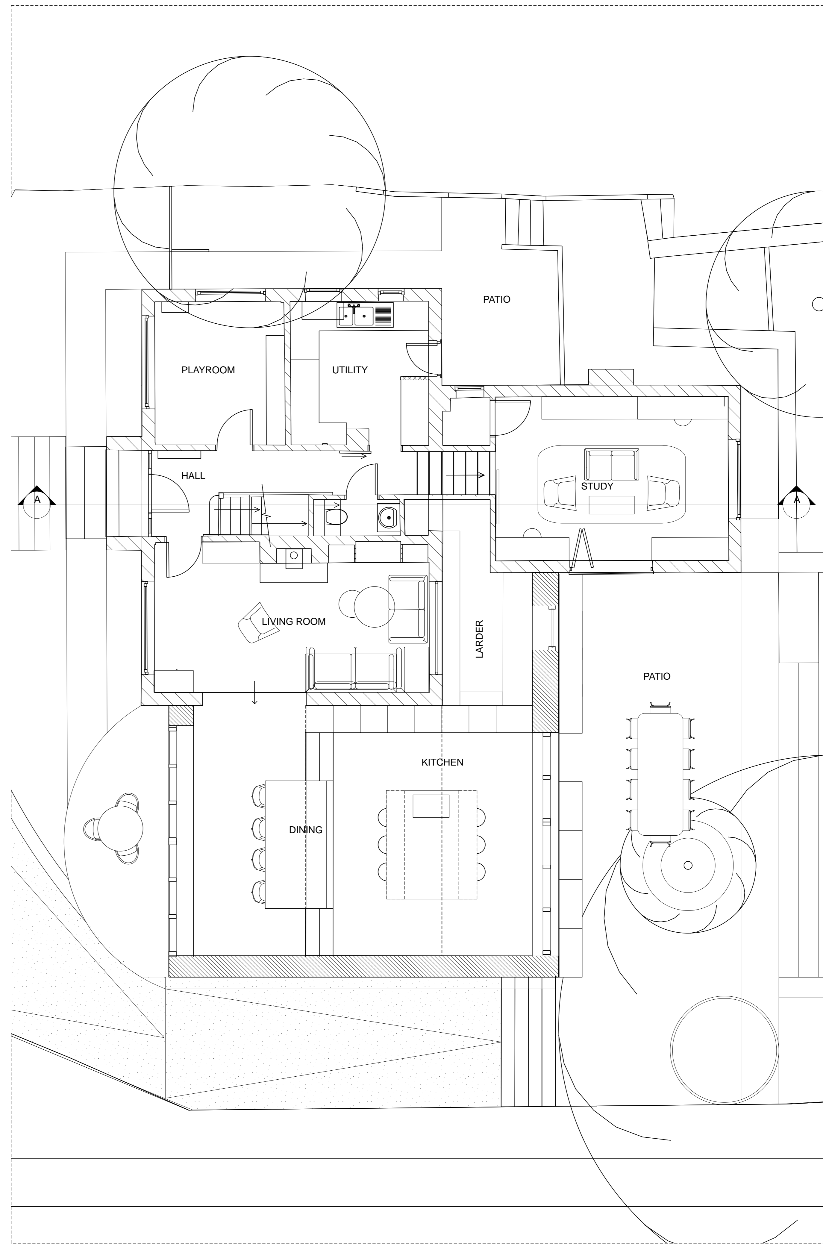
1 PROPOSED GROUND Scale: 1:50
