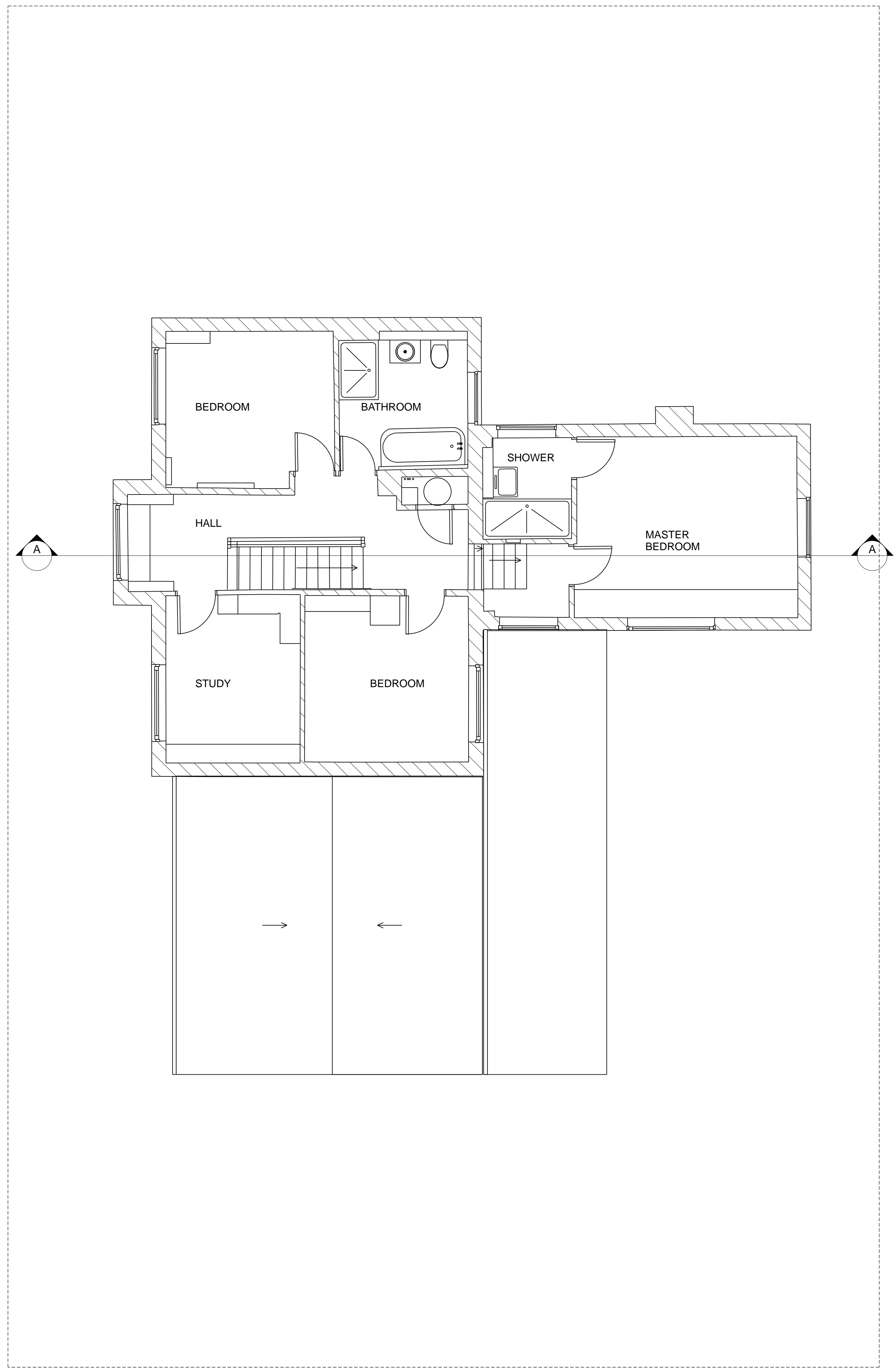
1 PROPOSED FIRST Scale: 1:50
