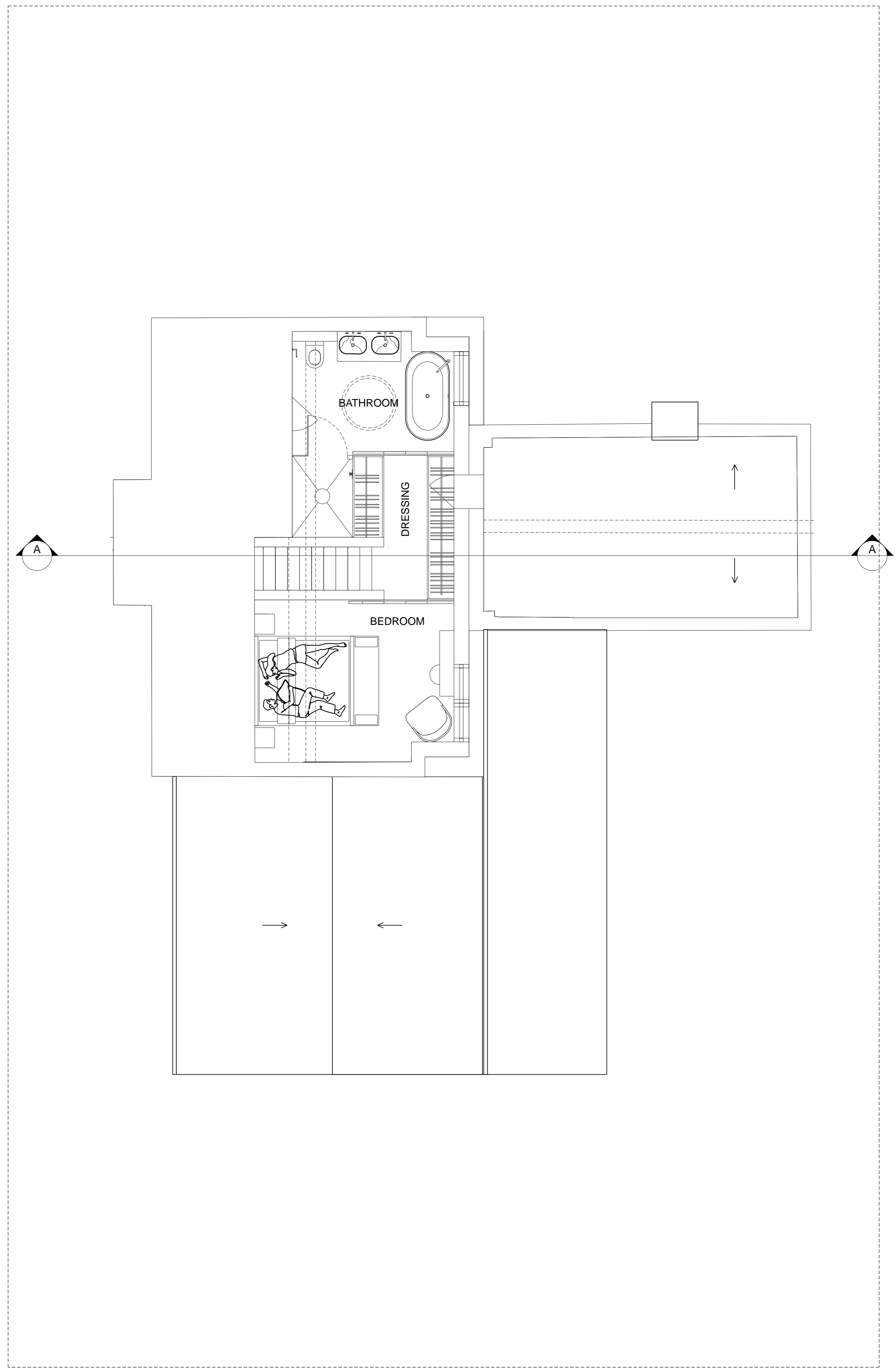
1 PROPOSED LOFT 1 Scale: 1:50
