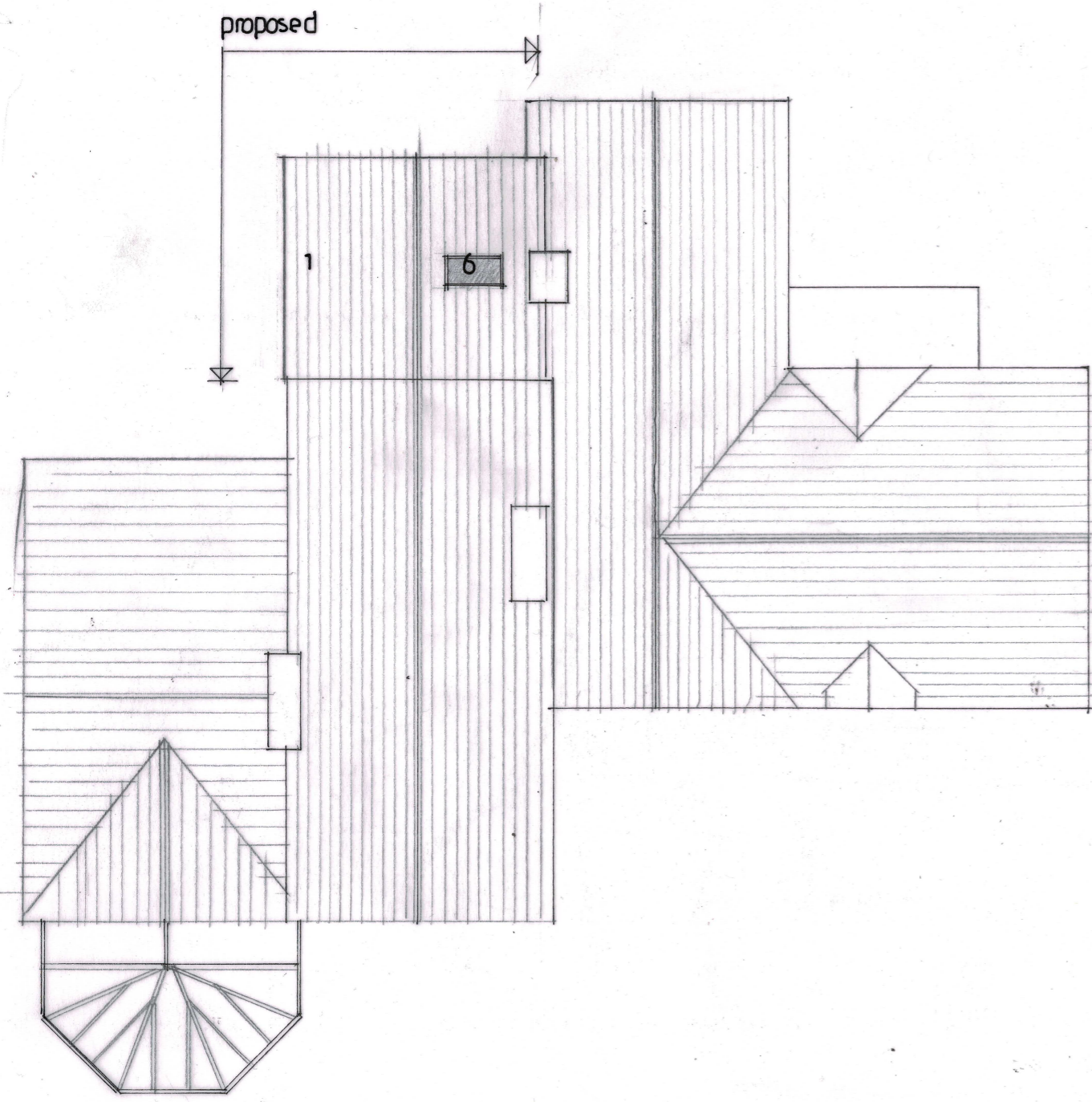
Roof Plan
