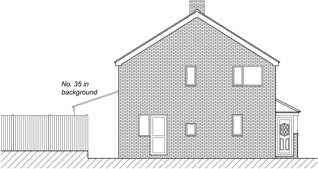
SNORTH WEST (SIDE) ELEVATION
