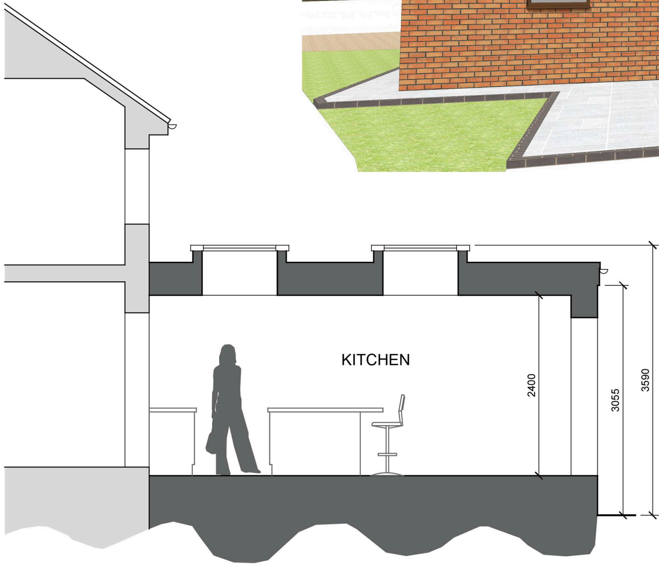
PROPOSED SECTION 1:50
