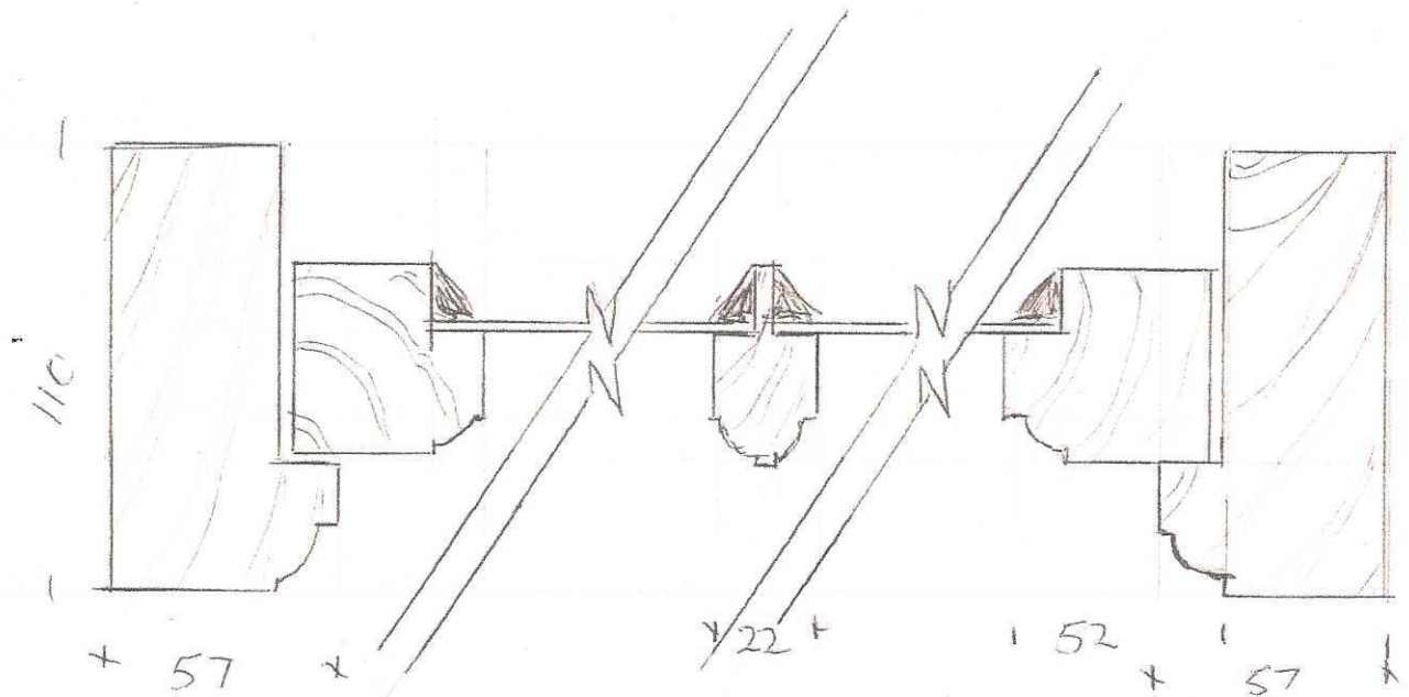
EXISTING WINDOW C
