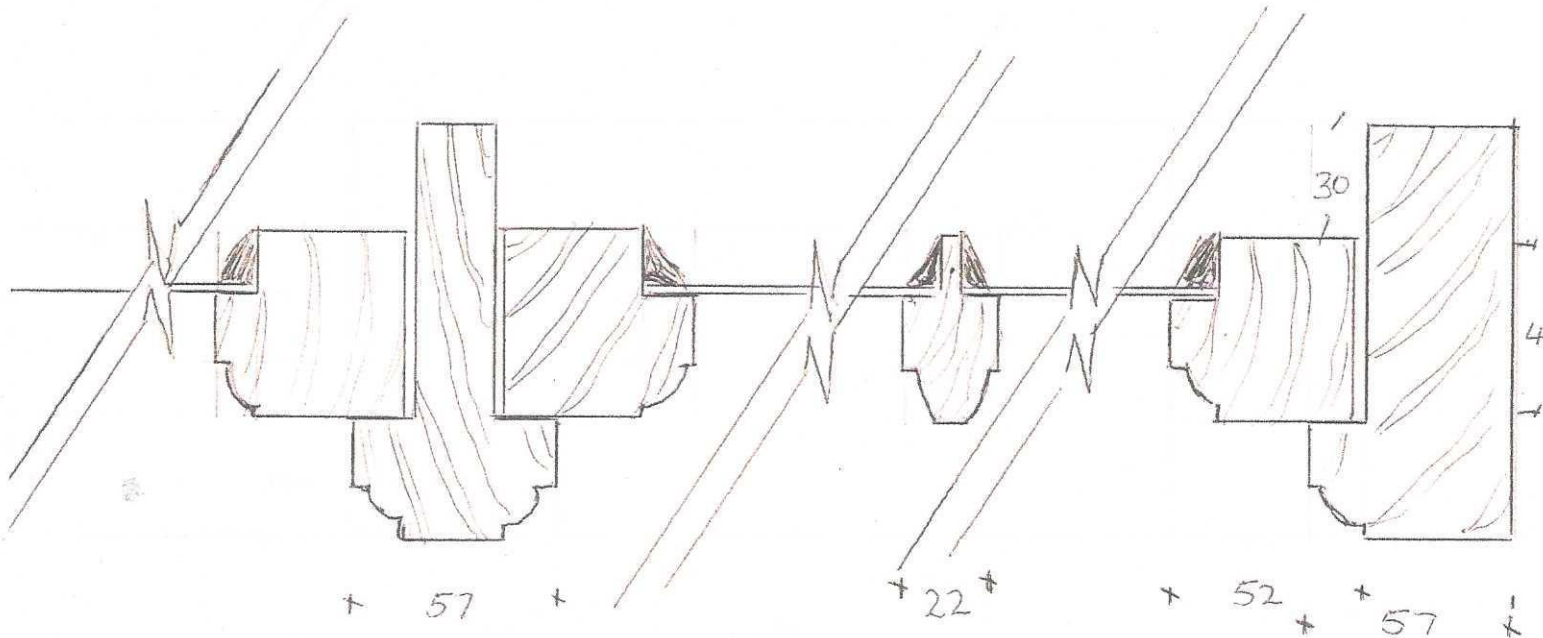
EXISTING WINDOW B + A & PROPOSED
