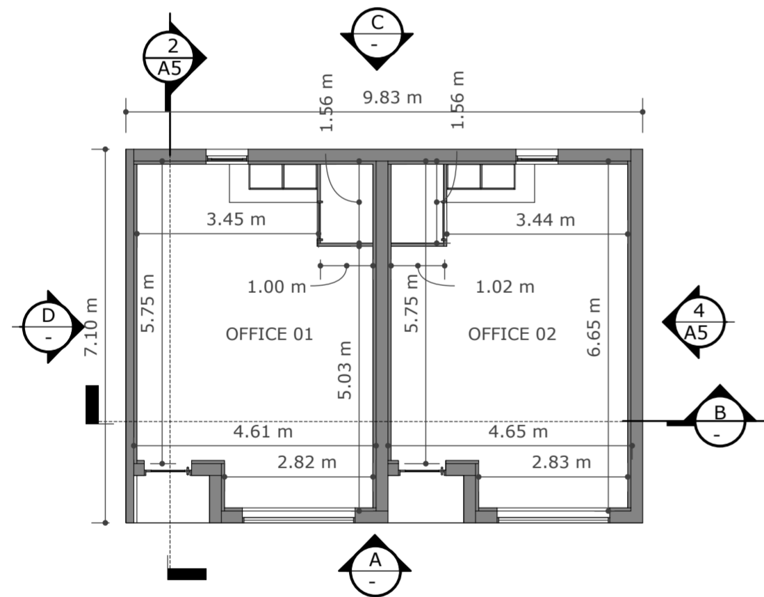
S A2 FLOOR PLAN 1:100
