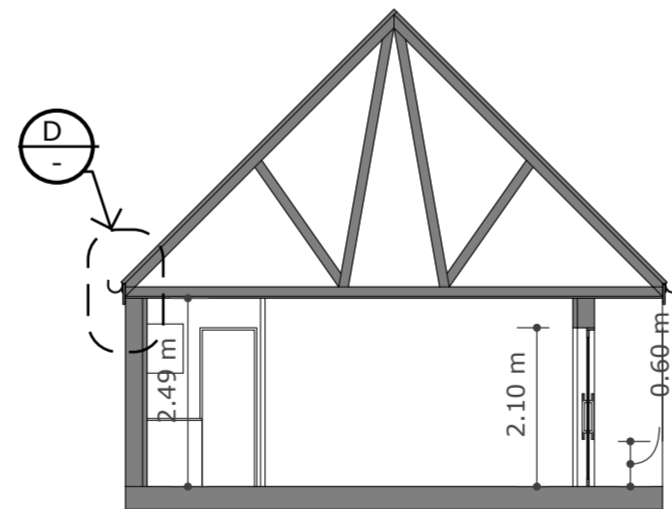
Z A2 SECTION Y-Y 1:100
