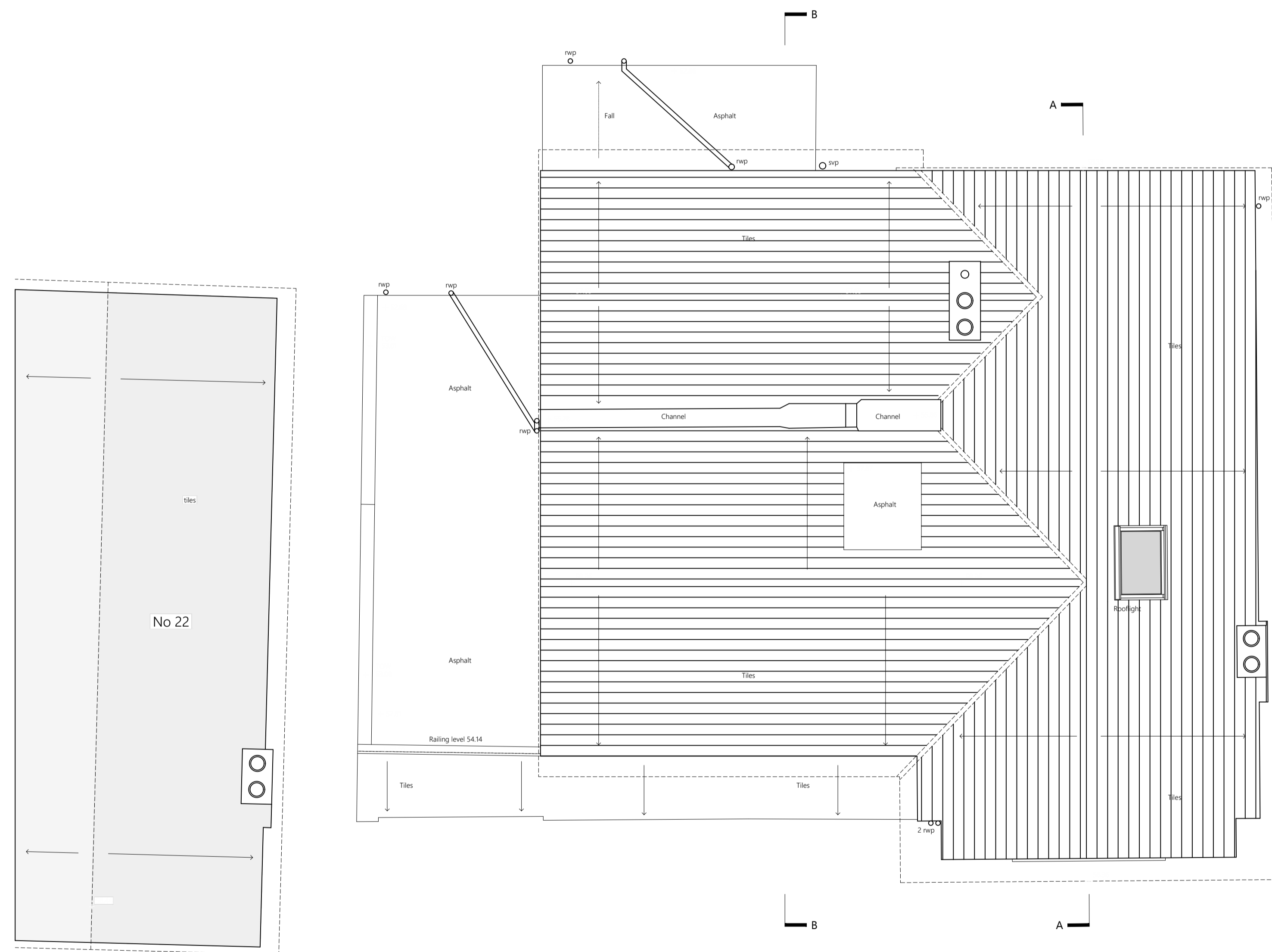
EXISTING ROOF Scale 1:50
