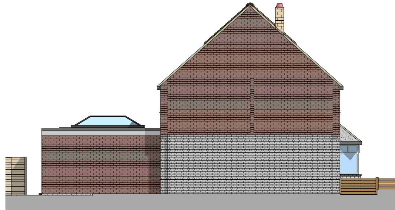
Proposed Side 02 Elevation Scale: 1:100
