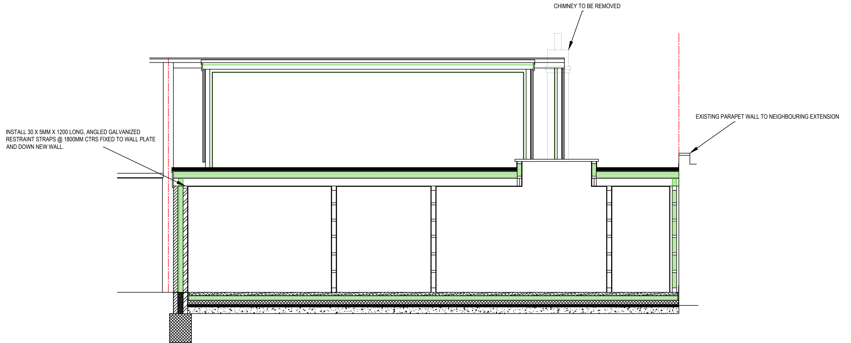
PROPOSED EXTENSION SECTION (REAR TO FRONT)
