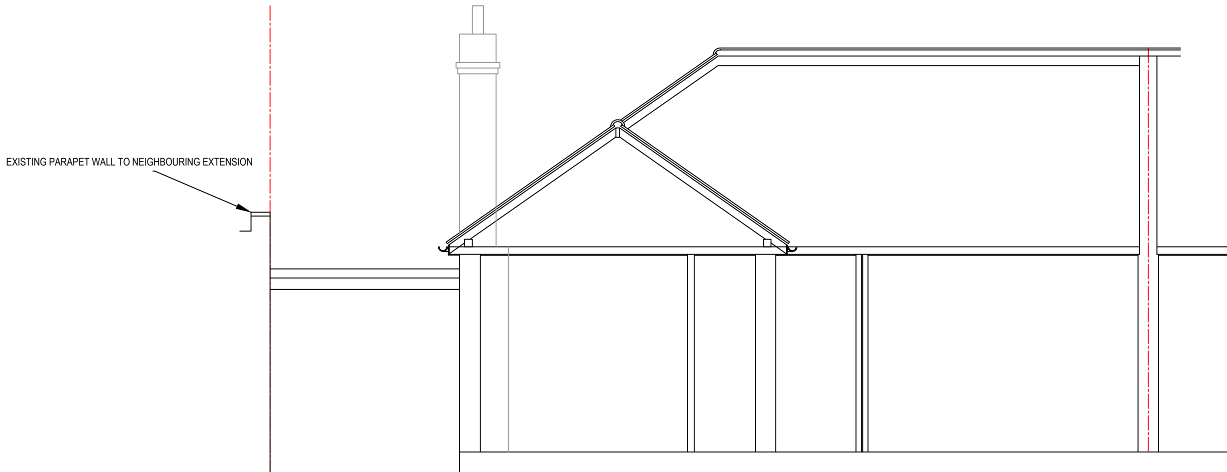
EXISTING SECTION (FRONT TO REAR)
