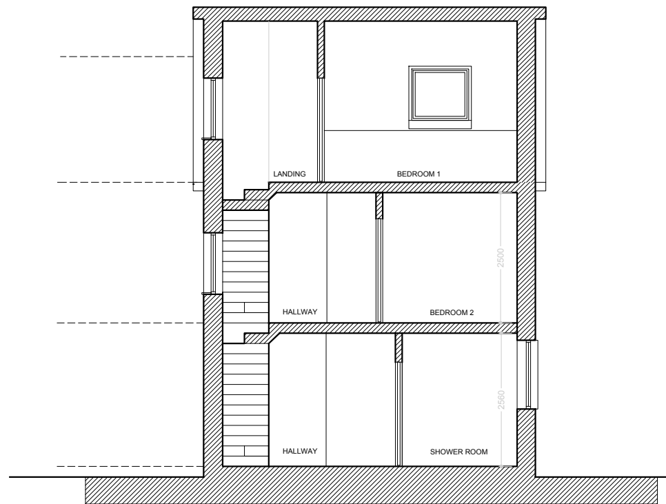
HOUSE TYPE "A" PROPOSED SECTION B-B
