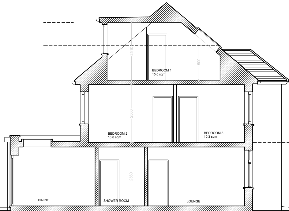
HOUSE TYPE "A" PROPOSED SECTION A-A
