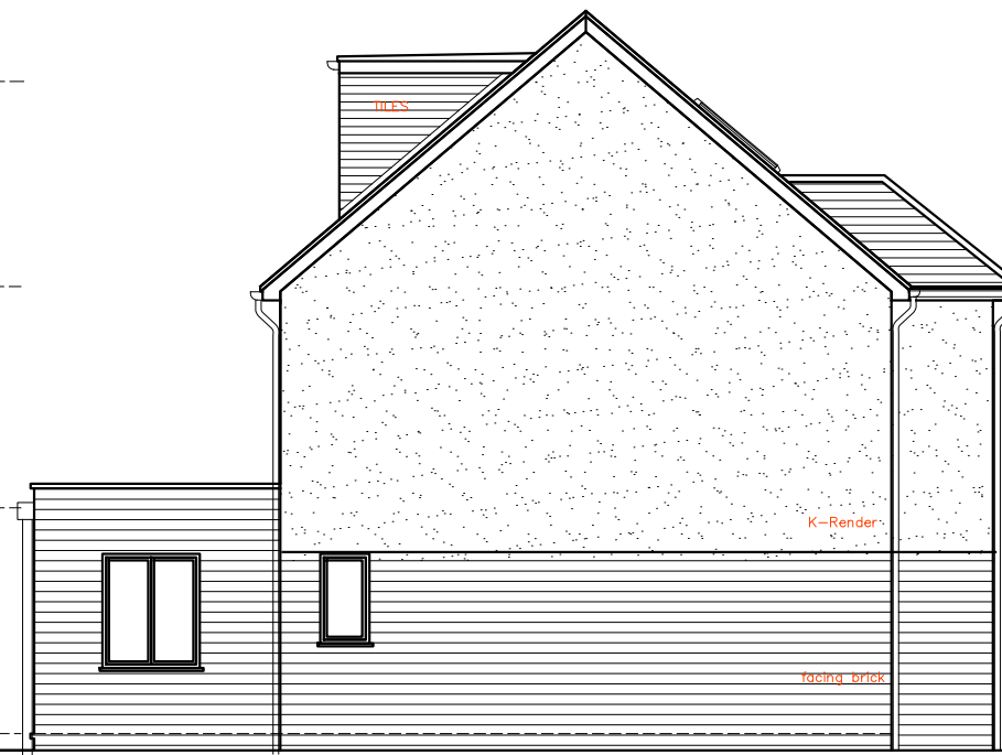
HOUSE TYPE "A" PROPOSED LEFT-SIDE ELEVATION
