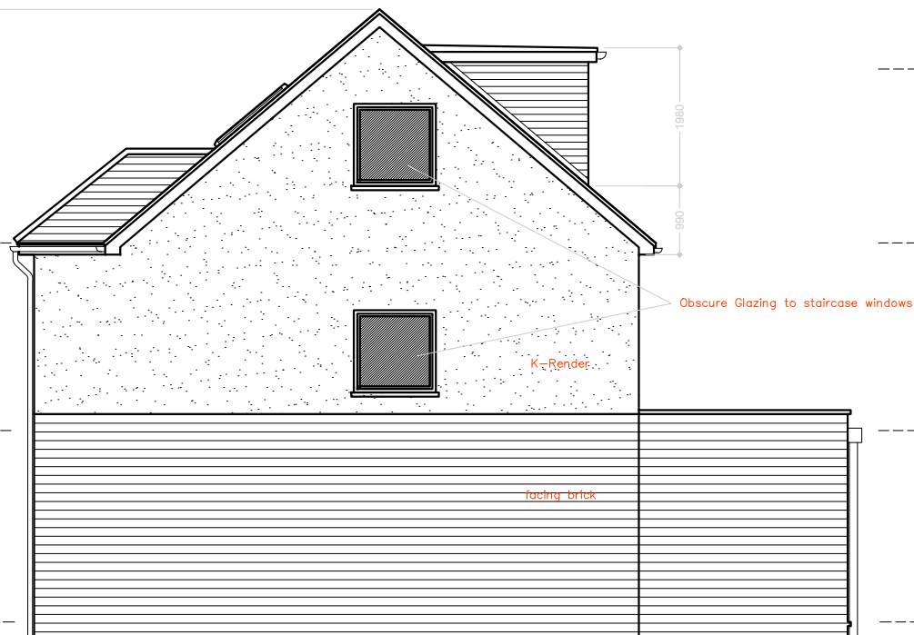
HOUSE TYPE "A" PROPOSED RIGHT -SIDE ELEVATION
