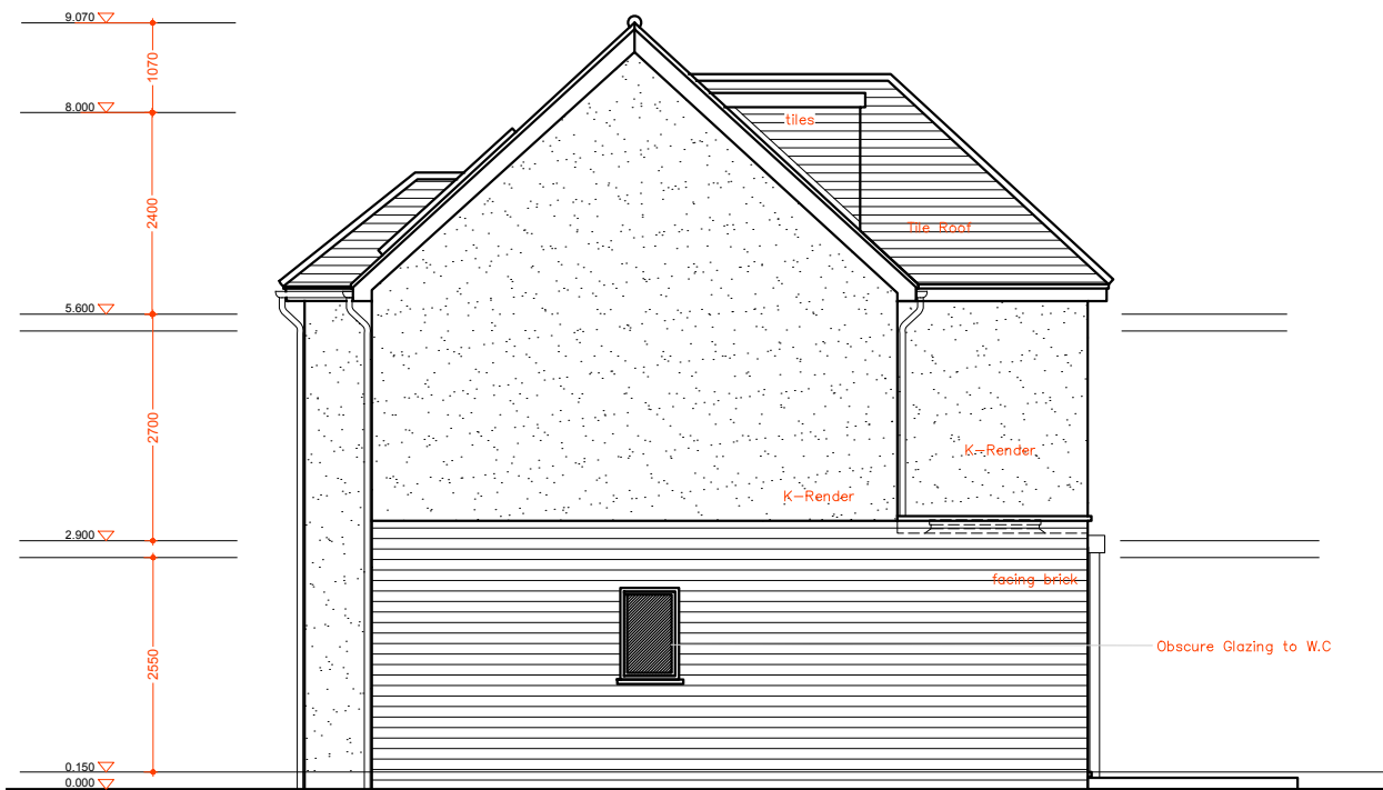
HOUSE TYPE "B" PROPOSED RIGHT -SIDE ELEVATION
