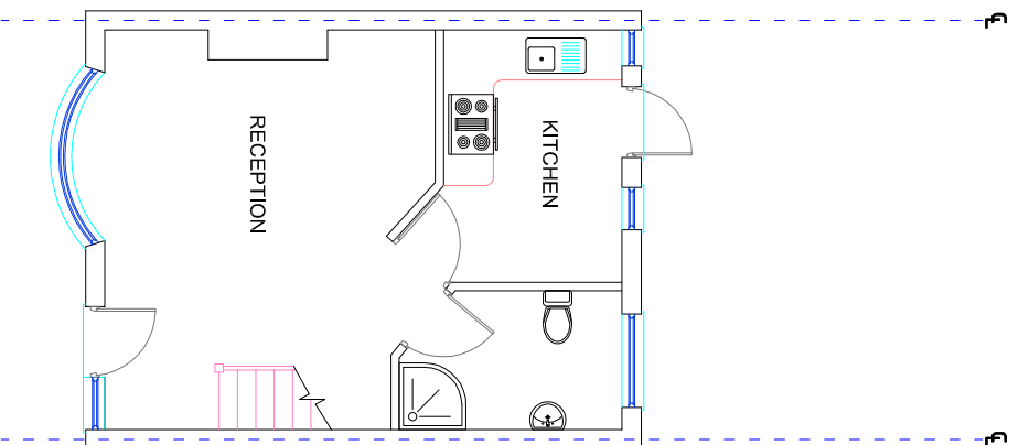
EXISTING GROUND FLOOR PLAN
