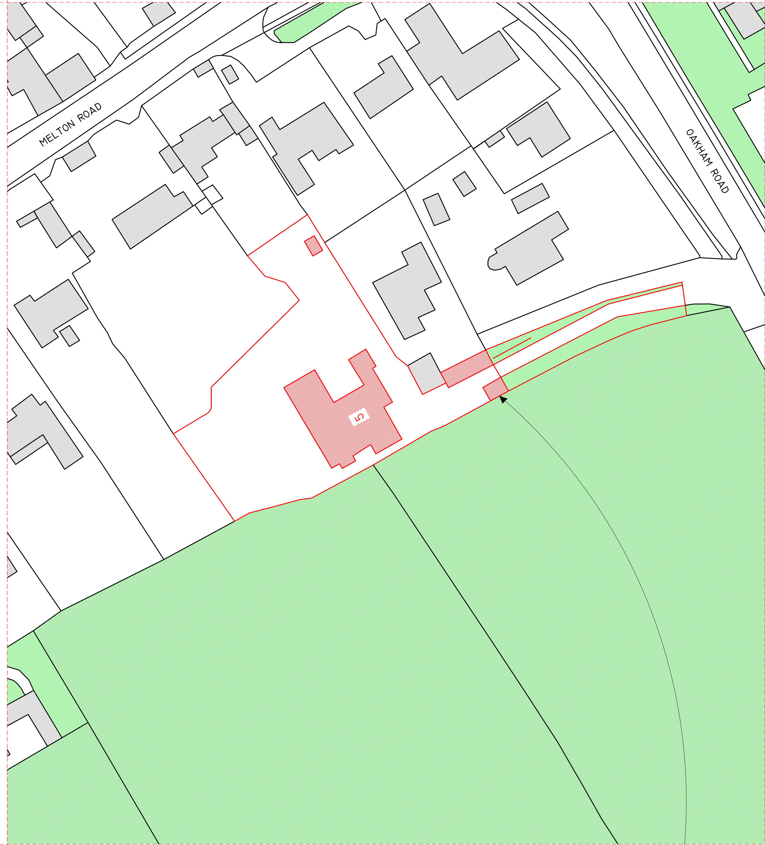
BLOCK PLAN OF THE SITE, EXISTING PLAN, SCALE 1:500
