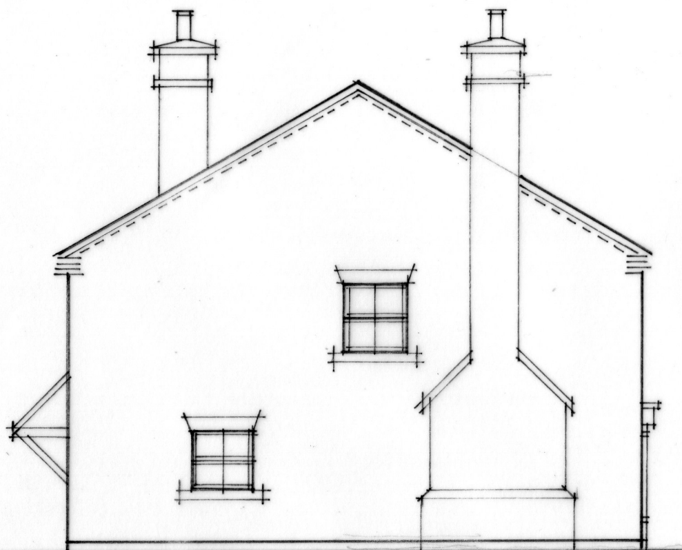
SIDE ELEVATION SOUTH EAST
