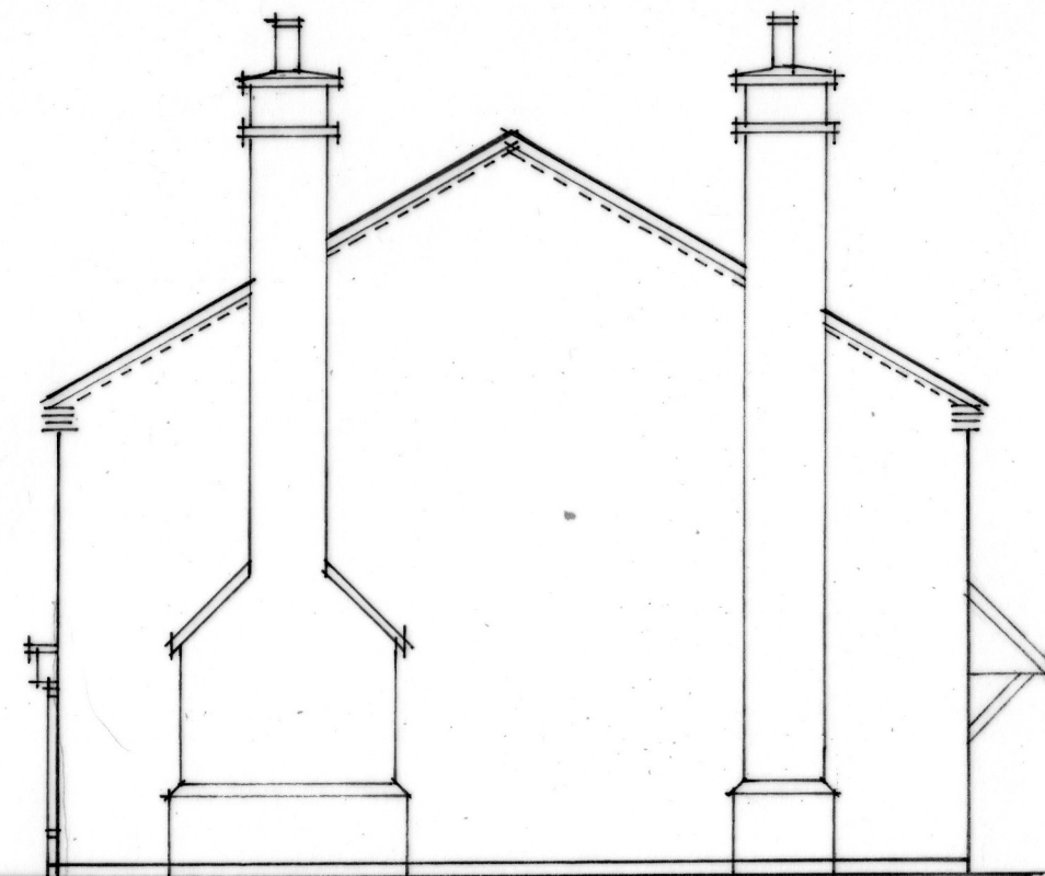
SIDE ELEVATION NORTH WEST
