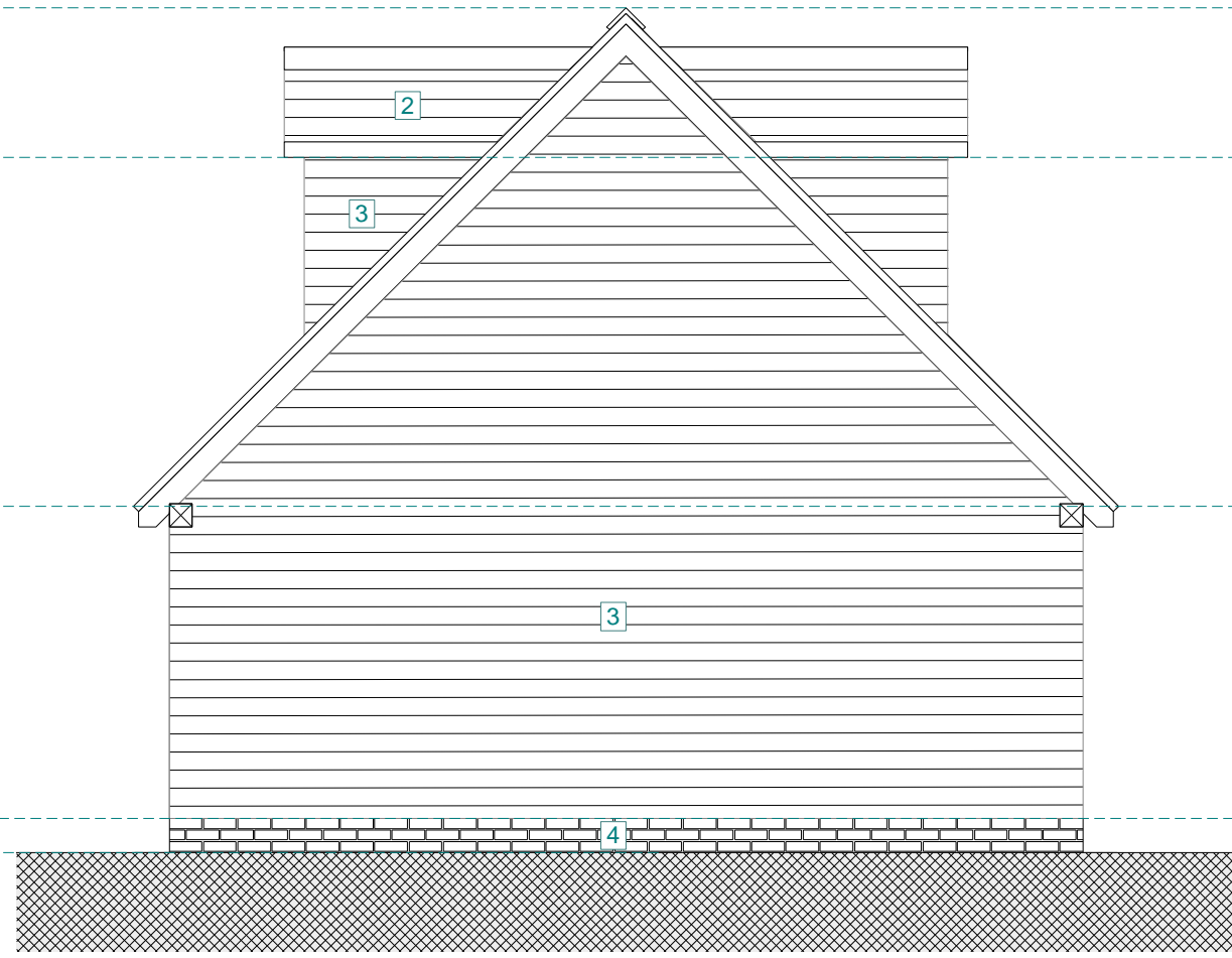
001 | Proposed North Elevation 1:50
