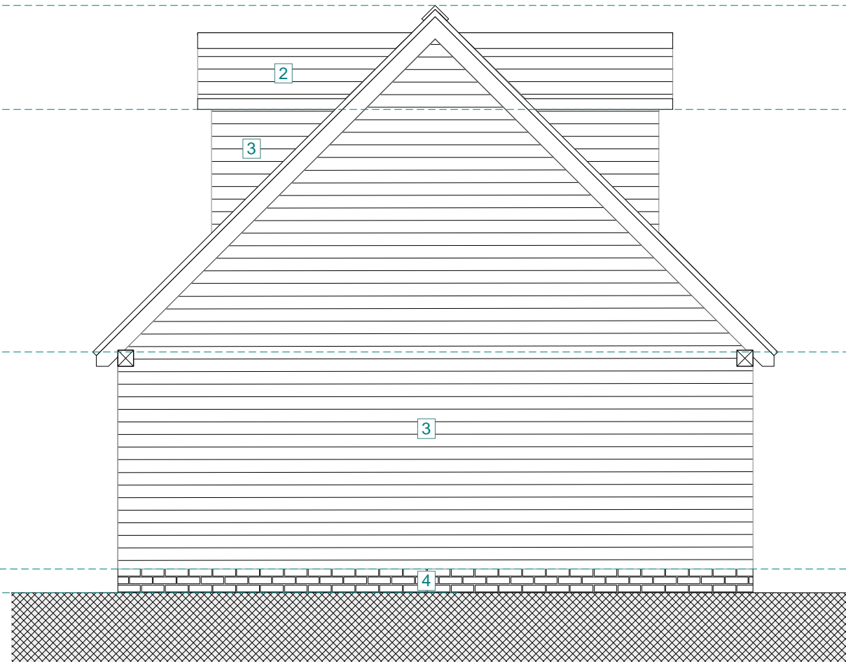
001 Existing North Elevation 1:50
