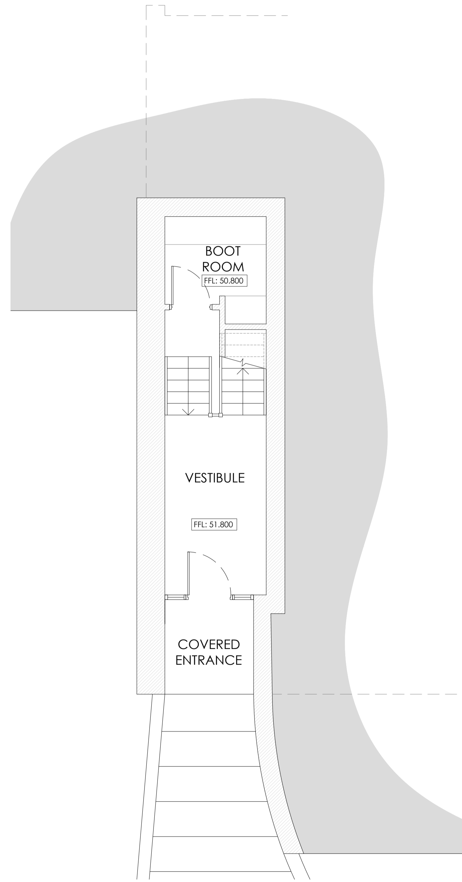
LOWER GROUND FLOOR PLAN 1:50
