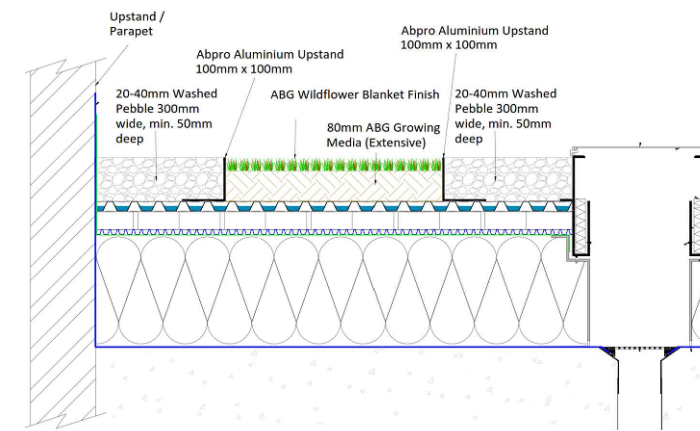
2 Green Roof Build-up Detail 1:20 @ A3
