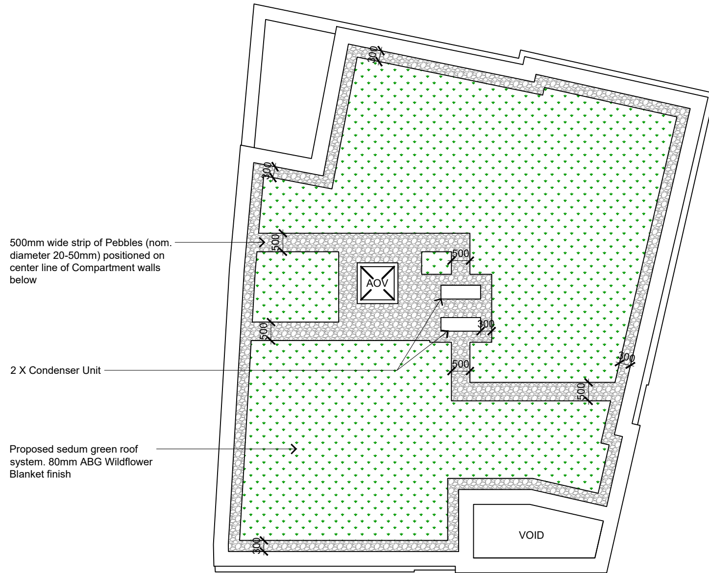
1 Proposed Roof Plan 1:100 @ A3
