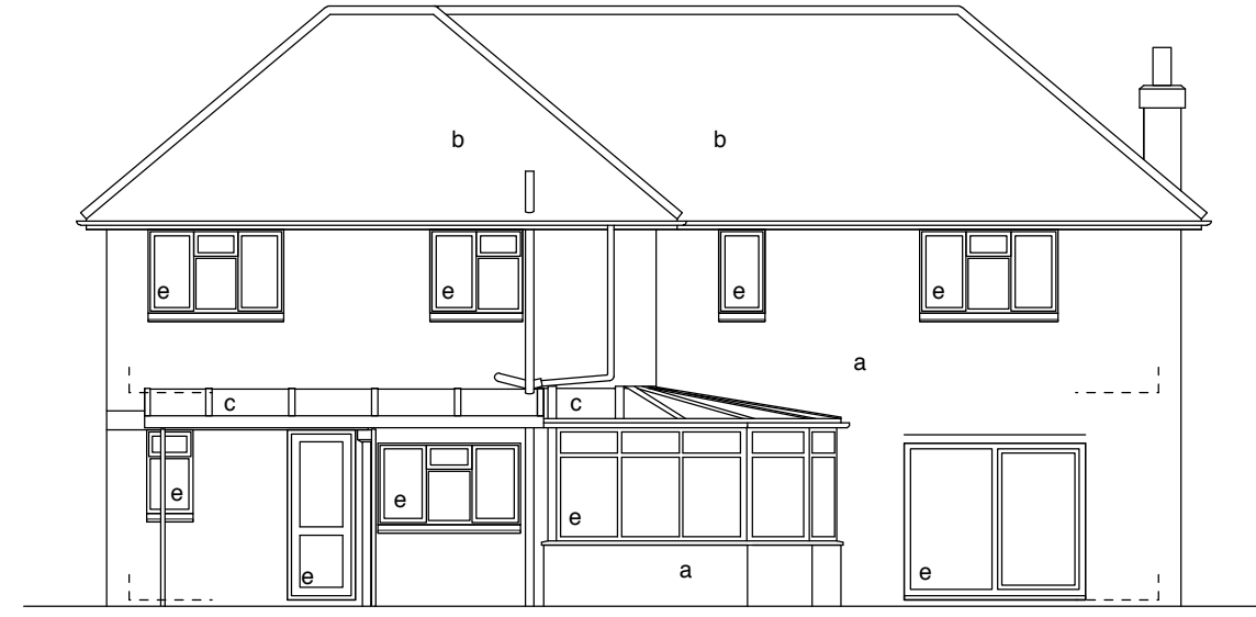
Rear (North) Elevation Existing
