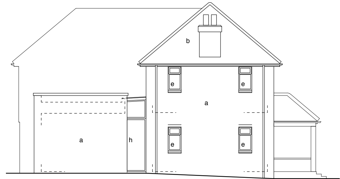
Side (West) Elevation Proposed
