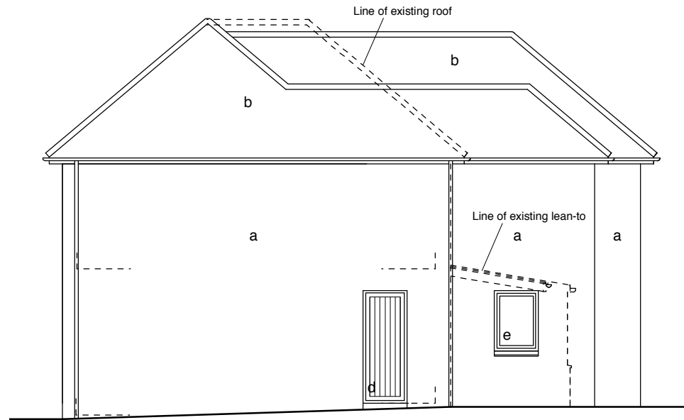
Side (East) Elevation Proposed
