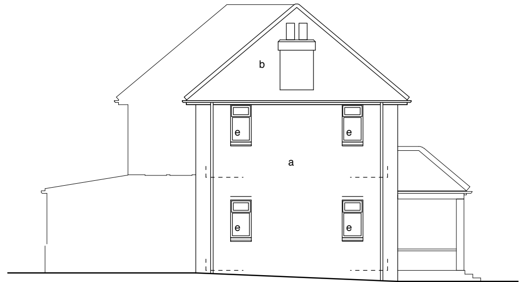
Side (West) Elevation Existing
