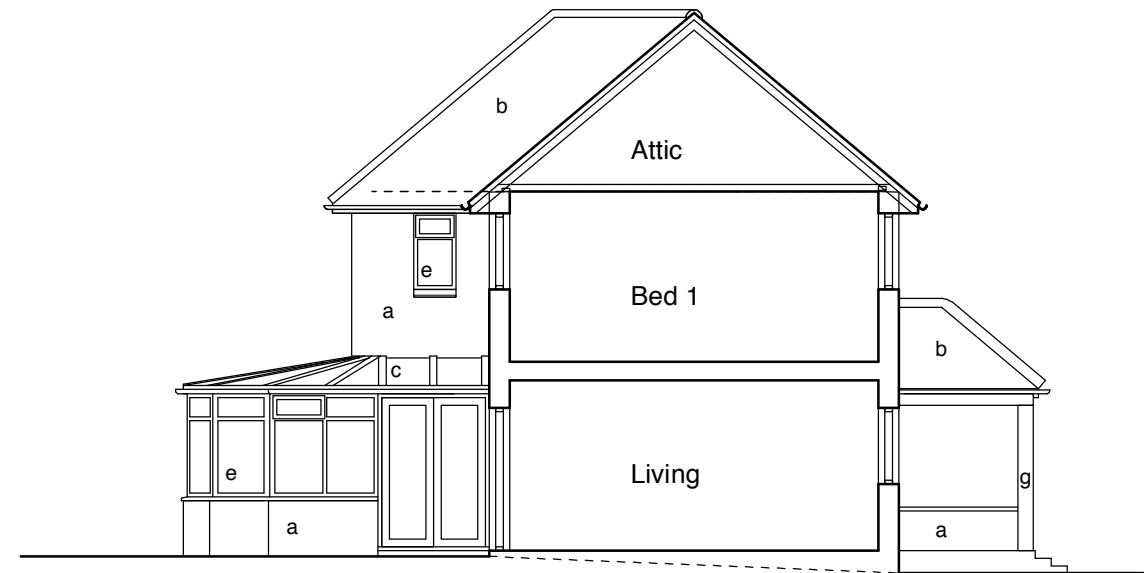
Section AA Existing
